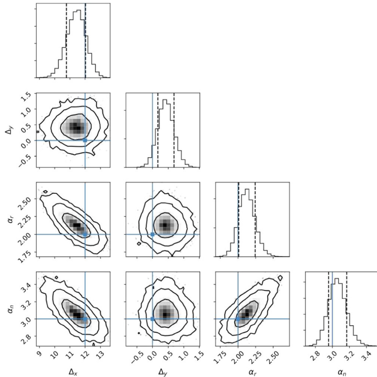
Figure 7. from Ofer Springer et al 2024 Astron. J. 167 doi:10.3847/1538-3881/ad408d https://dx.doi.org/10.3847/1538-3881/ad408d © 2024. The Author(s). Published by the American Astronomical Society.
