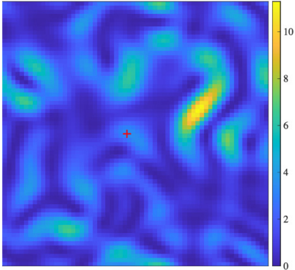
Transient statistic Z(x, y)^2
