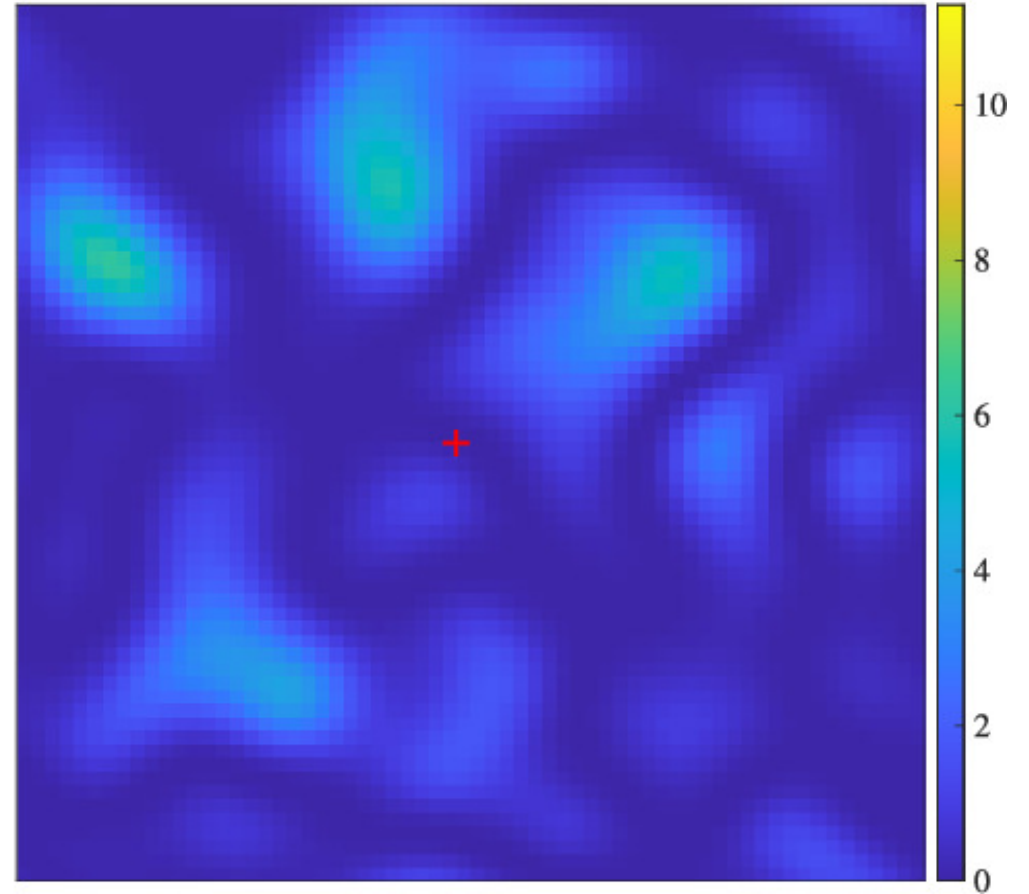
Proper statistic S(x, y)^2
