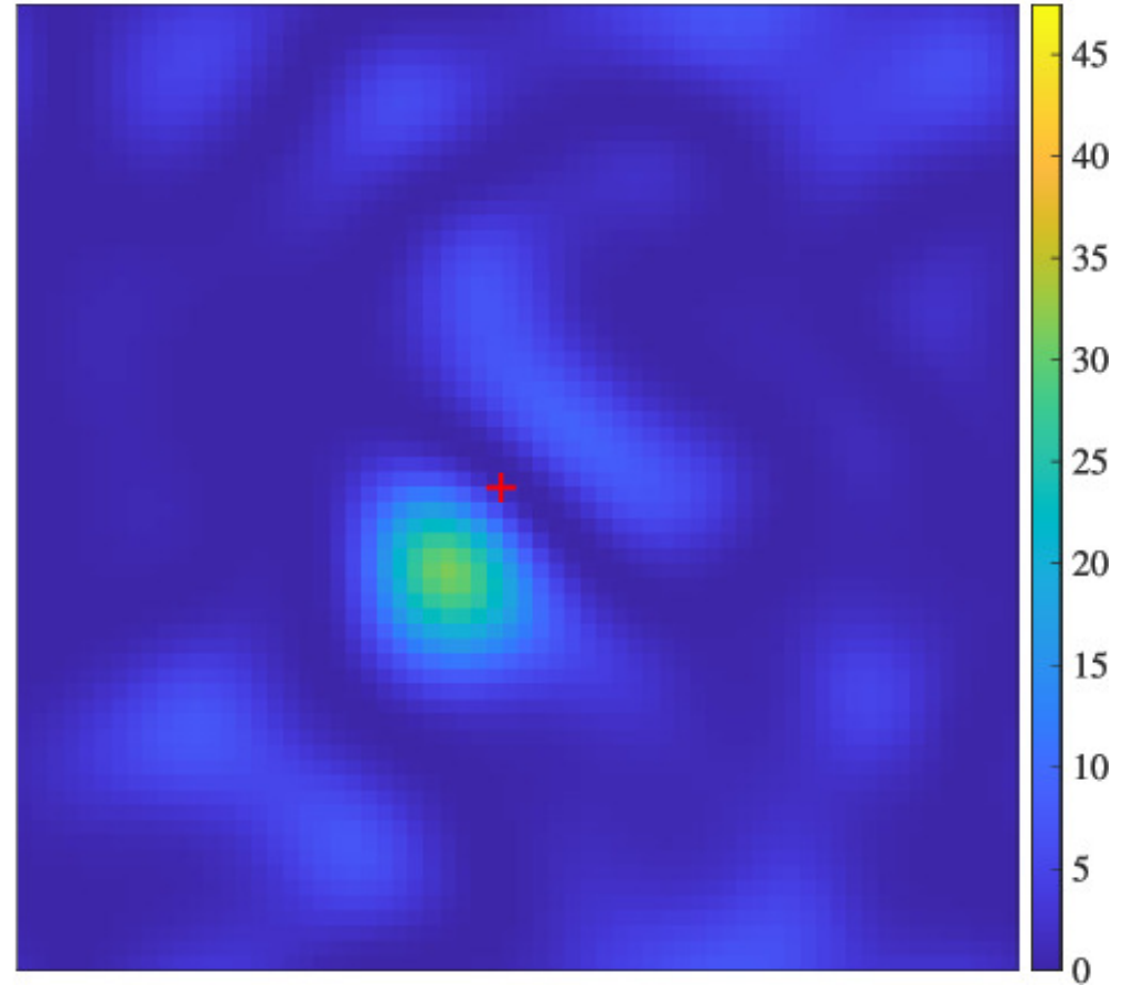
Proper statistic S(x, y)^2
