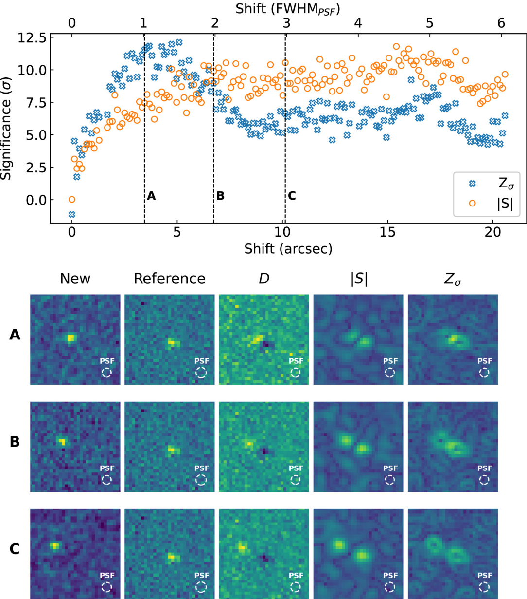
Figure 12. from Ofer Springer et al 2024 Astron. J. 167 doi:10.3847/1538-3881/ad408d https://dx.doi.org/10.3847/1538-3881/ad408d © 2024. The Author(s). Published by the American Astronomical Society.
