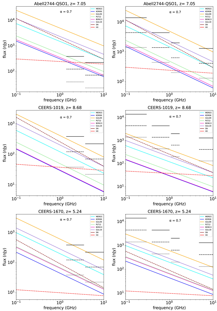
Figure A9. from Muhammad A. Latif et al 2024 Astron. J. 167 doi:10.3847/1538-3881/ad3b97 https://dx.doi.org/10.3847/1538-3881/ad3b97 © 2024. The Author(s). Published by the American Astronomical Society.
