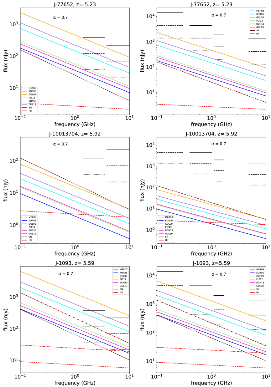
Figure A8. from Muhammad A. Latif et al 2024 Astron. J. 167 doi:10.3847/1538-3881/ad3b97 https://dx.doi.org/10.3847/1538-3881/ad3b97 © 2024. The Author(s). Published by the American Astronomical Society.
