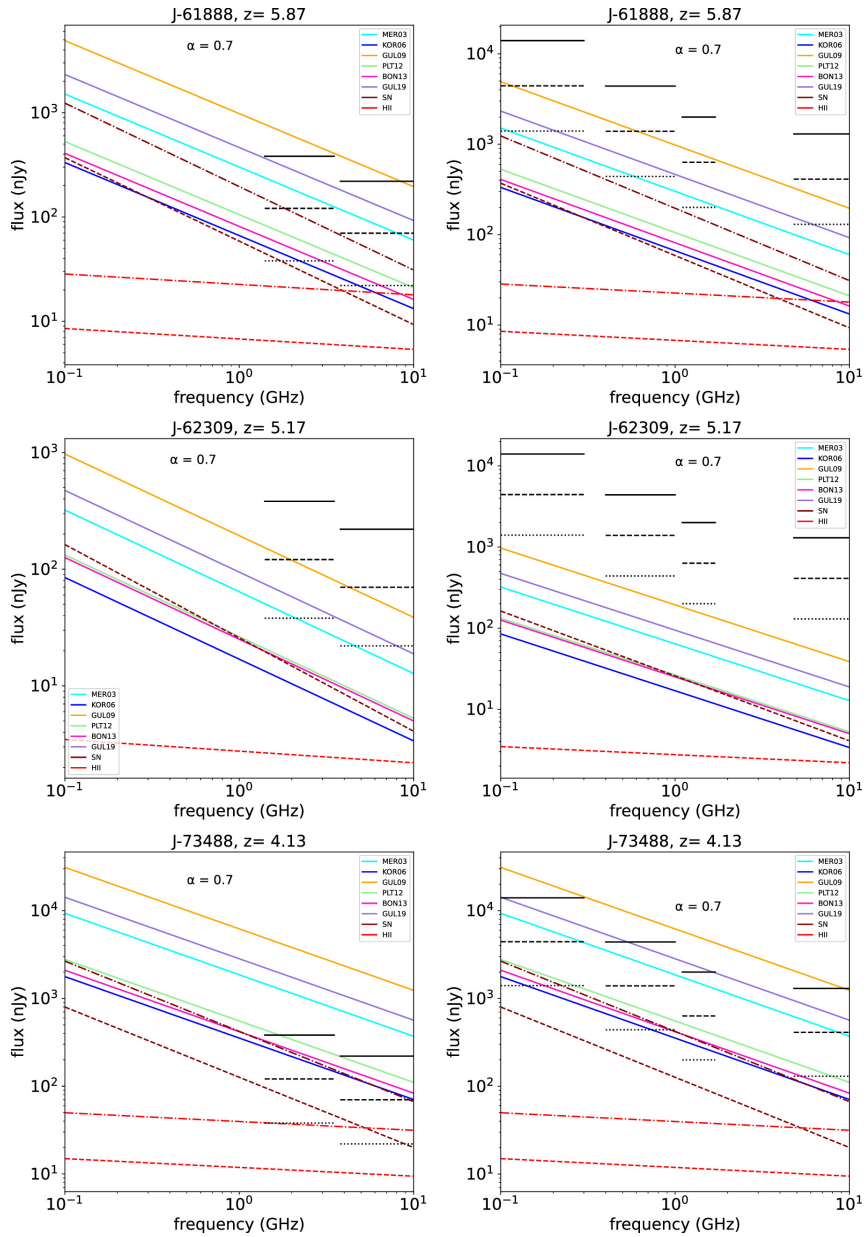
Figure A7. from Muhammad A. Latif et al 2024 Astron. J. 167 doi:10.3847/1538-3881/ad3b97 https://dx.doi.org/10.3847/1538-3881/ad3b97 © 2024. The Author(s). Published by the American Astronomical Society.
