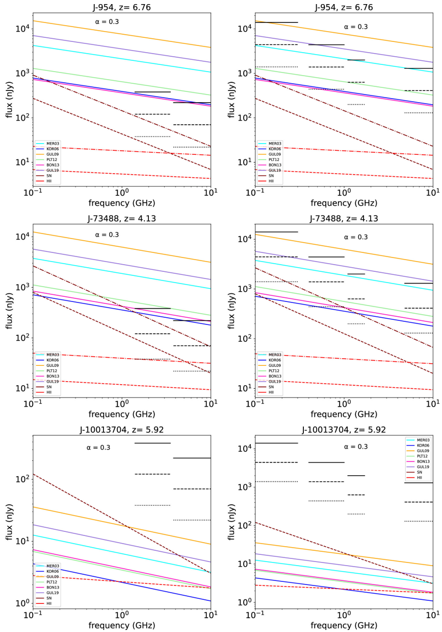
Figure 1. from Muhammad A. Latif et al 2024 Astron. J. 167 doi:10.3847/1538-3881/ad3b97 https://dx.doi.org/10.3847/1538-3881/ad3b97 © 2024. The Author(s). Published by the American Astronomical Society.
