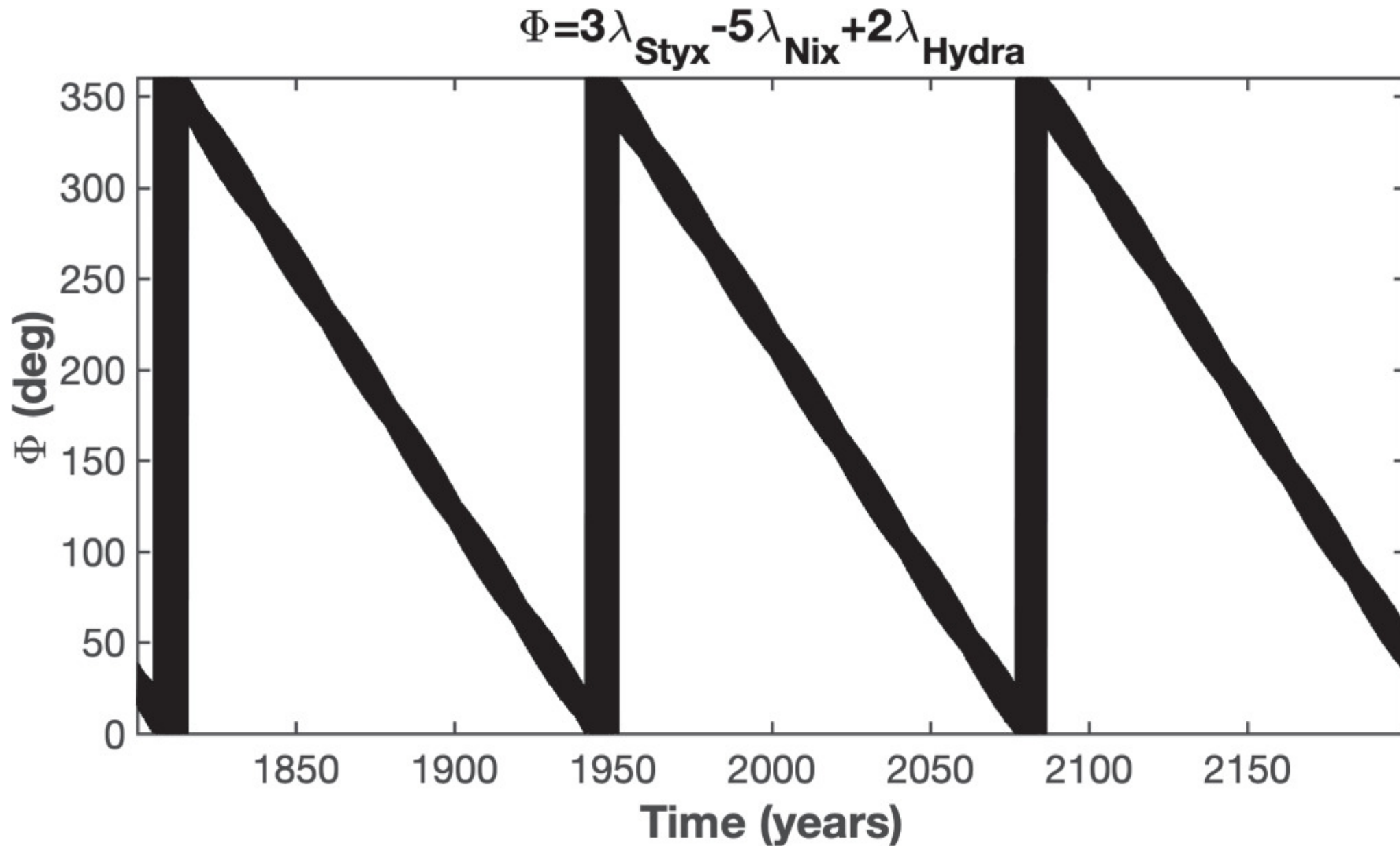
Figure 9. from Marina Brozovi and Robert A. Jacobson 2024 Astron. J. 167 doi:10.3847/1538-3881/ad39f0 https://dx.doi.org/10.3847/1538-3881/ad39f0 © 2024. The Author(s). Published by the American Astronomical Society.
