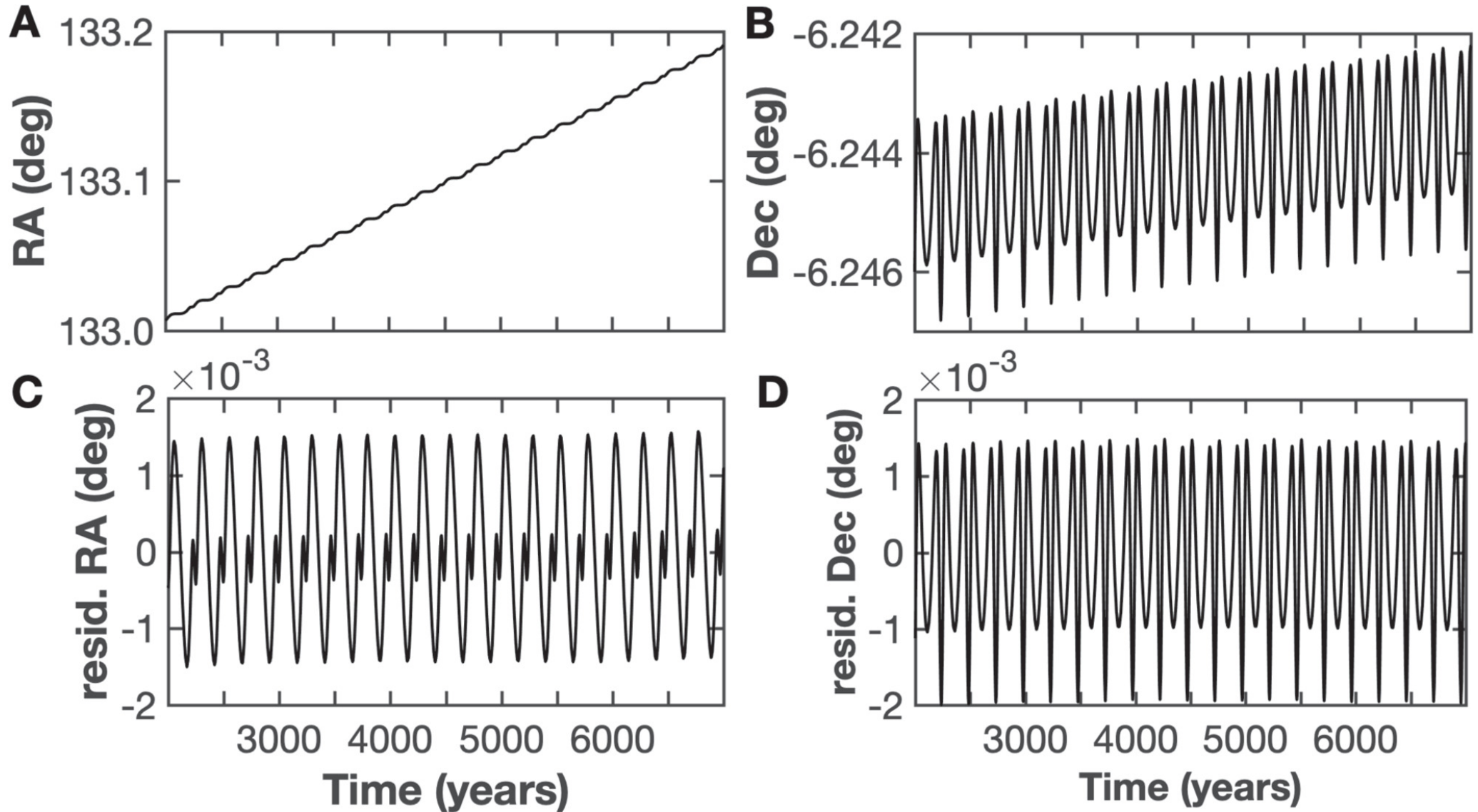
Figure 7. from Marina Brozovi and Robert A. Jacobson 2024 Astron. J. 167 doi:10.3847/1538-3881/ad39f0 https://dx.doi.org/10.3847/1538-3881/ad39f0 © 2024. The Author(s). Published by the American Astronomical Society.
