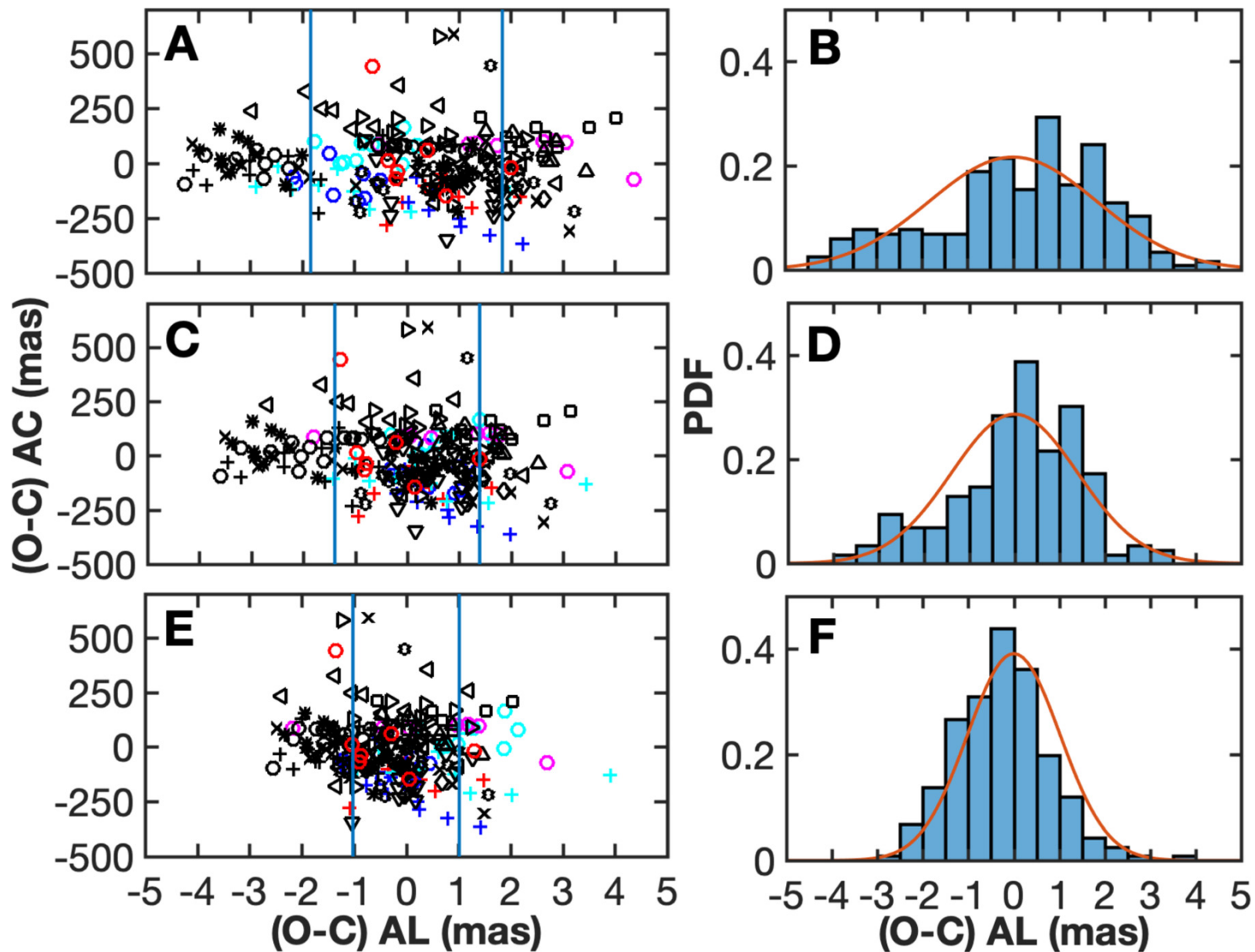
Figure 3. from Marina Brozovi and Robert A. Jacobson 2024 Astron. J. 167 doi:10.3847/1538-3881/ad39f0 https://dx.doi.org/10.3847/1538-3881/ad39f0 © 2024. The Author(s). Published by the American Astronomical Society.
