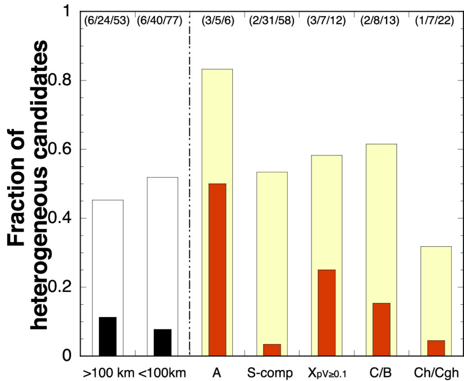
Figure 8. from Sunao Hasegawa et al 2024 Astron. J. 167 doi:10.3847/1538-3881/ad3045 https://dx.doi.org/10.3847/1538-3881/ad3045 © 2024. The Author(s). Published by the American Astronomical Society.
