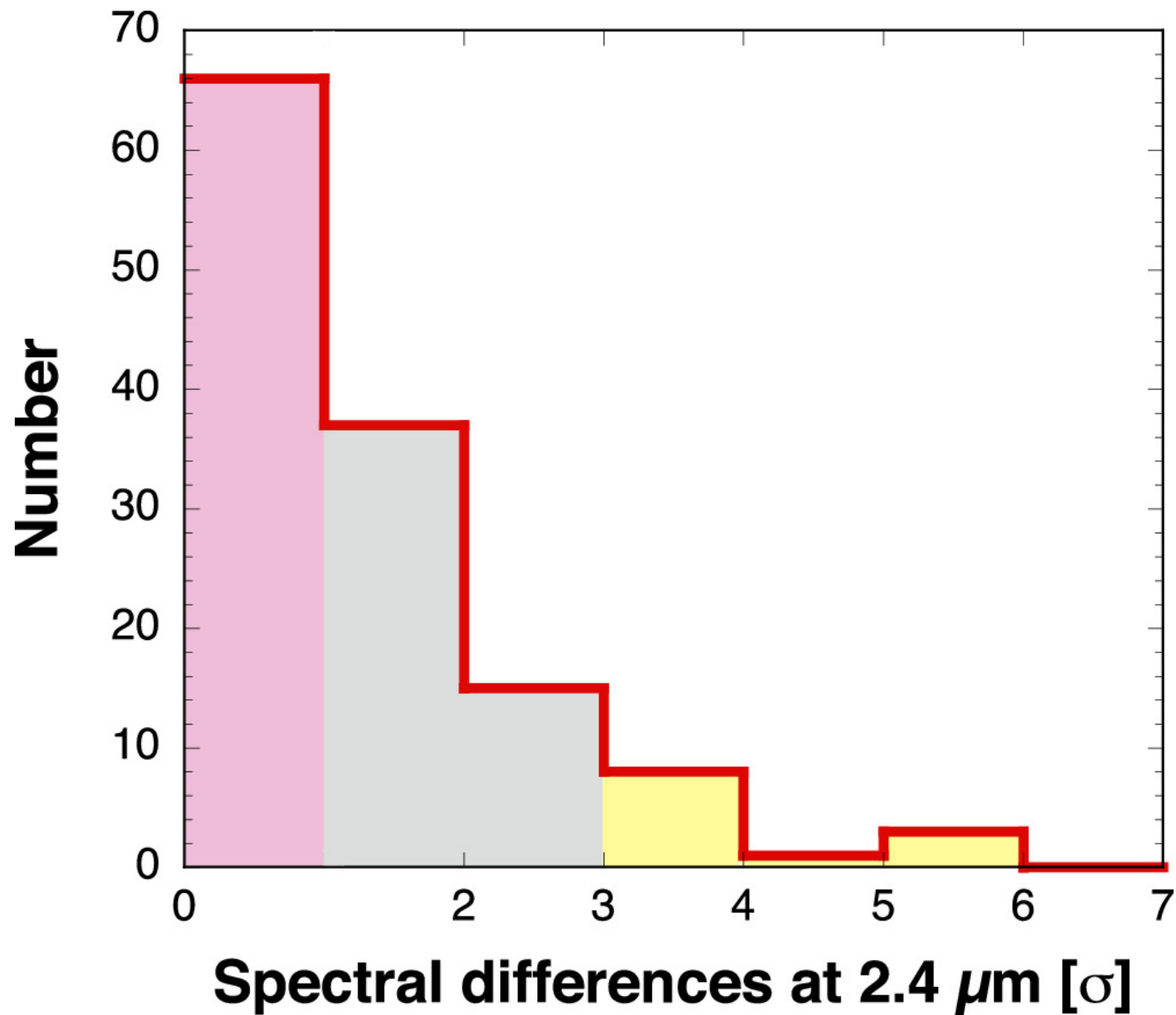
Figure 6. from Sunao Hasegawa et al 2024 Astron. J. 167 doi:10.3847/1538-3881/ad3045 https://dx.doi.org/10.3847/1538-3881/ad3045 © 2024. The Author(s). Published by the American Astronomical Society.
