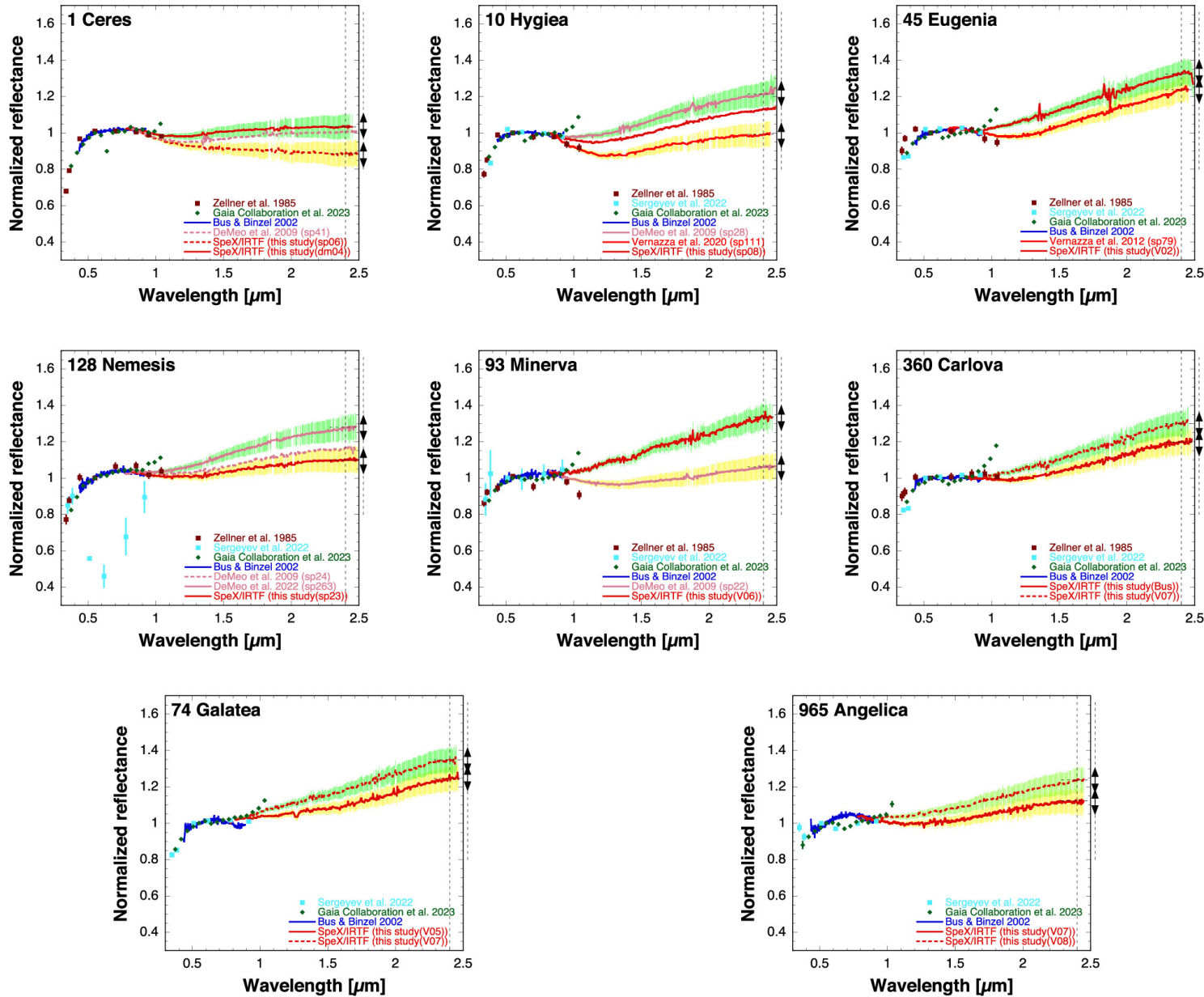
Figure 5. from Sunao Hasegawa et al 2024 Astron. J. 167 doi:10.3847/1538-3881/ad3045 https://dx.doi.org/10.3847/1538-3881/ad3045 © 2024. The Author(s). Published by the American Astronomical Society.
