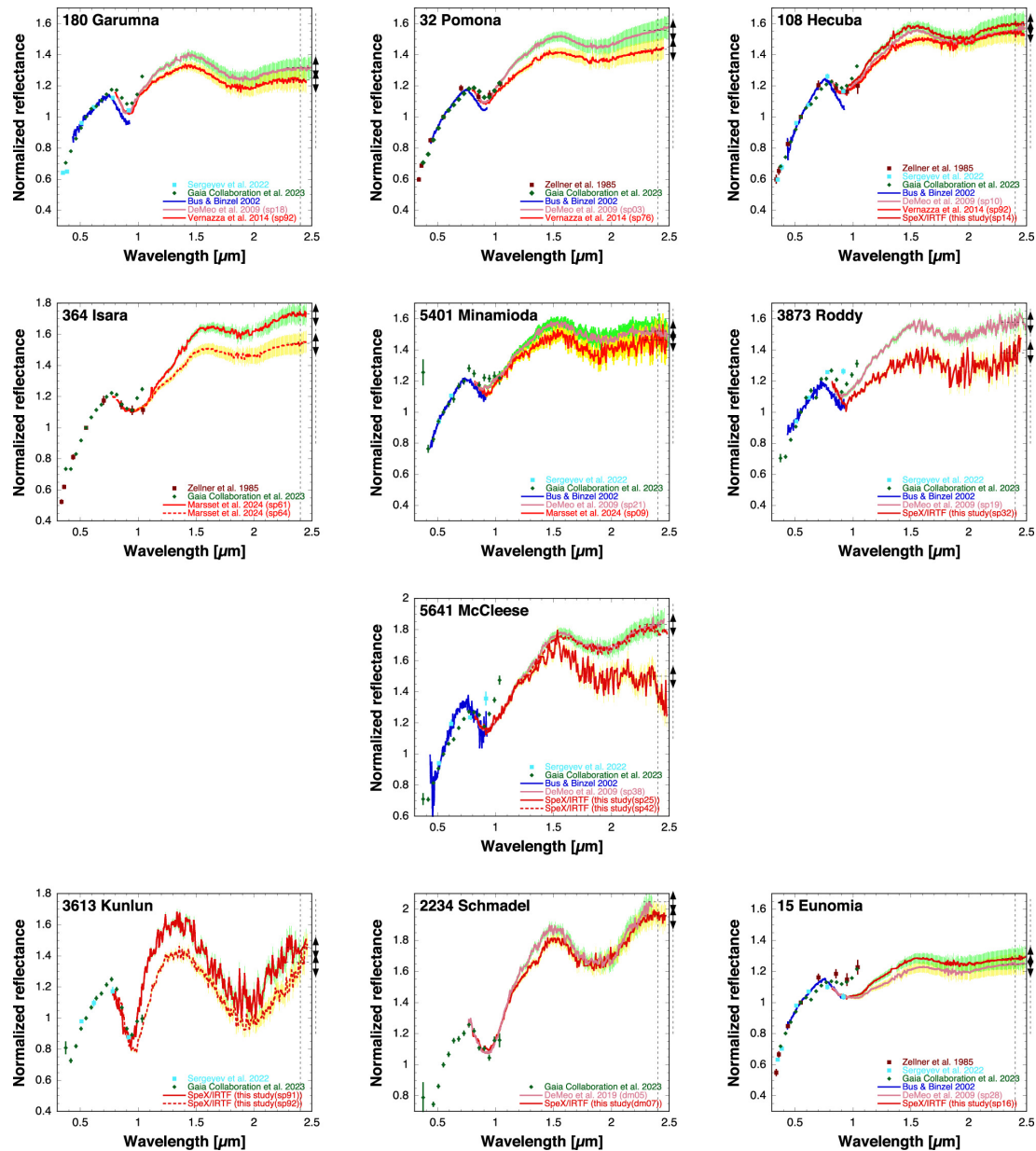
Figure 2. from Sunao Hasegawa et al 2024 Astron. J. 167 doi:10.3847/1538-3881/ad3045 https://dx.doi.org/10.3847/1538-3881/ad3045 © 2024. The Author(s). Published by the American Astronomical Society.
