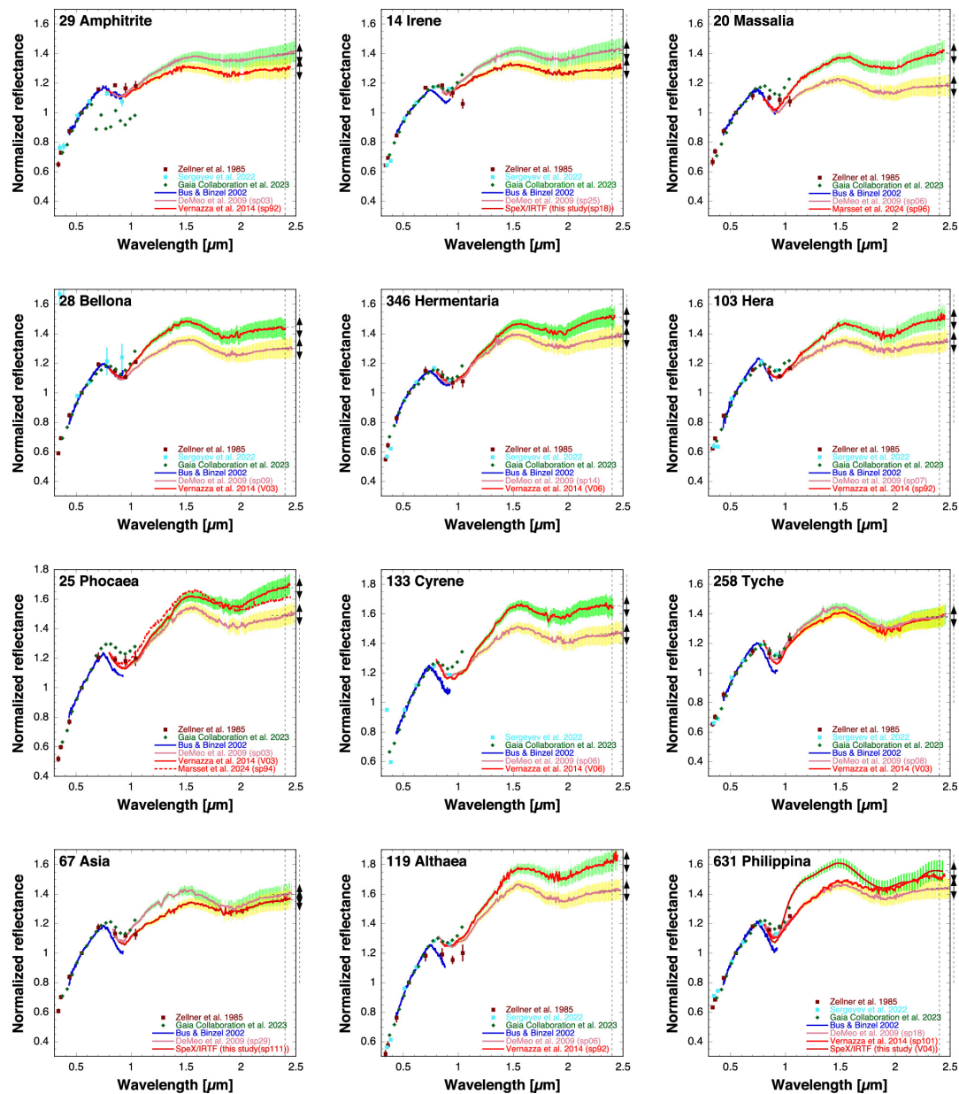
Figure 2. from Sunao Hasegawa et al 2024 Astron. J. 167 doi:10.3847/1538-3881/ad3045 https://dx.doi.org/10.3847/1538-3881/ad3045 © 2024. The Author(s). Published by the American Astronomical Society.
