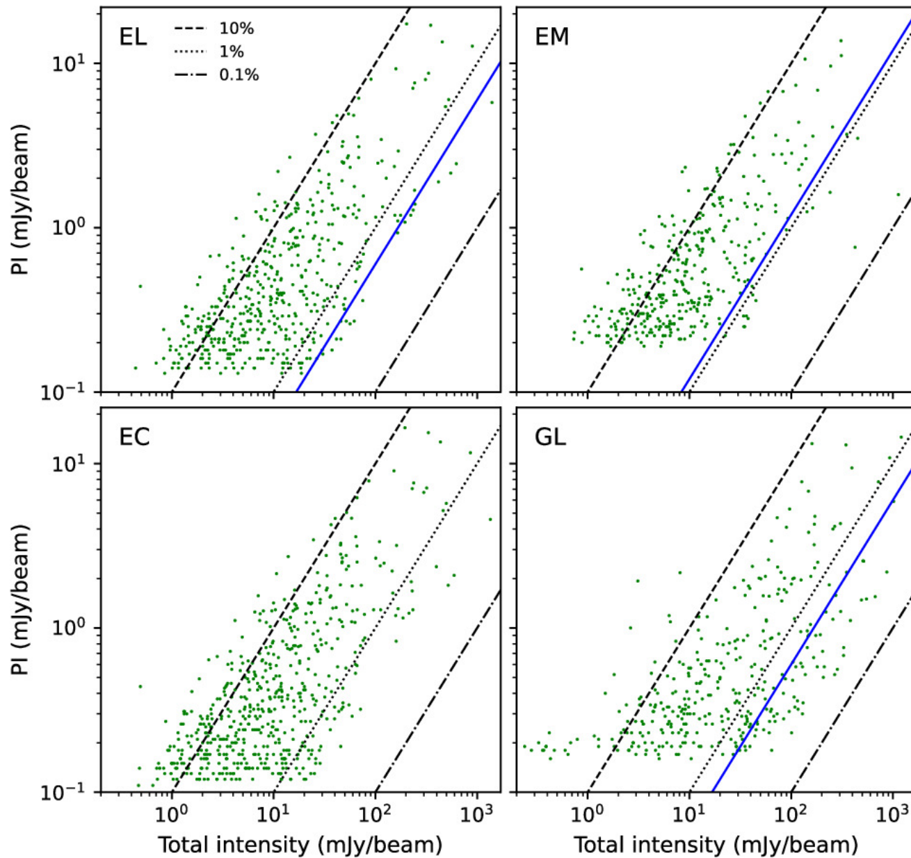
Figure 8. from S. Vanderwoude et al 2024 Astron. J. 167 doi:10.3847/1538-3881/ad2fc8 https://dx.doi.org/10.3847/1538-3881/ad2fc8 © 2024. The Author(s). Published by the American Astronomical Society.
