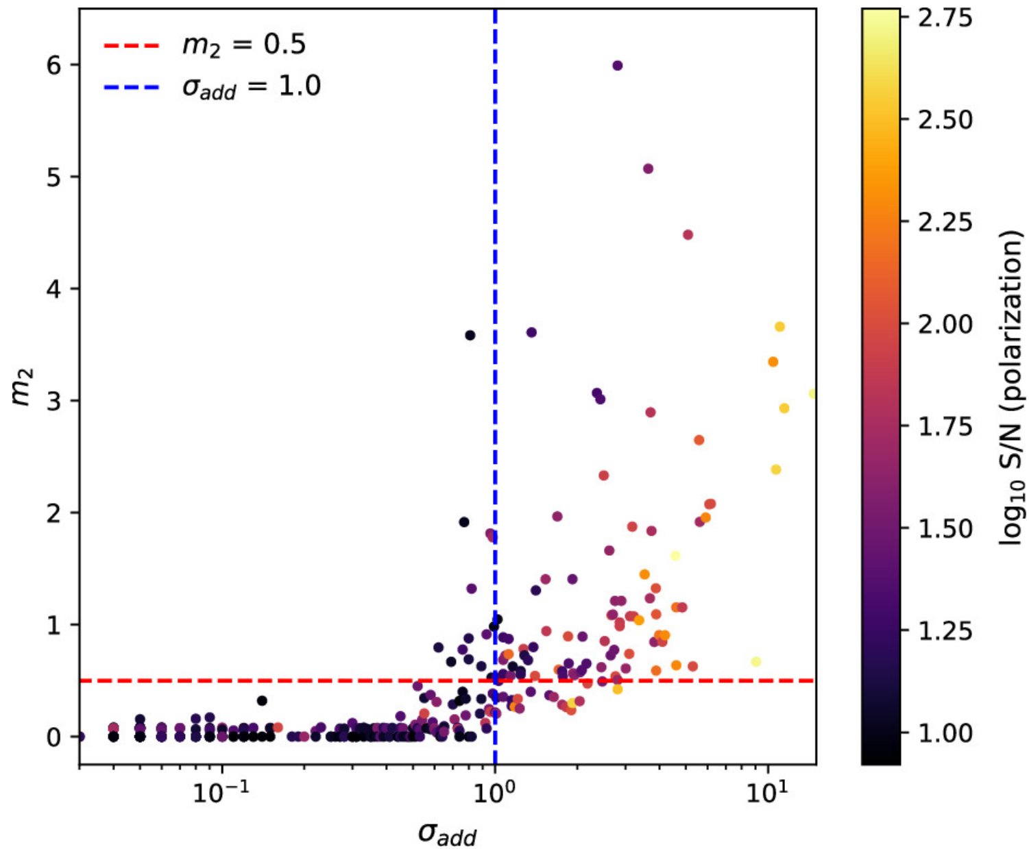
Figure 7. from S. Vanderwoude et al 2024 Astron. J. 167 doi:10.3847/1538-3881/ad2fc8 https://dx.doi.org/10.3847/1538-3881/ad2fc8 © 2024. The Author(s). Published by the American Astronomical Society.
