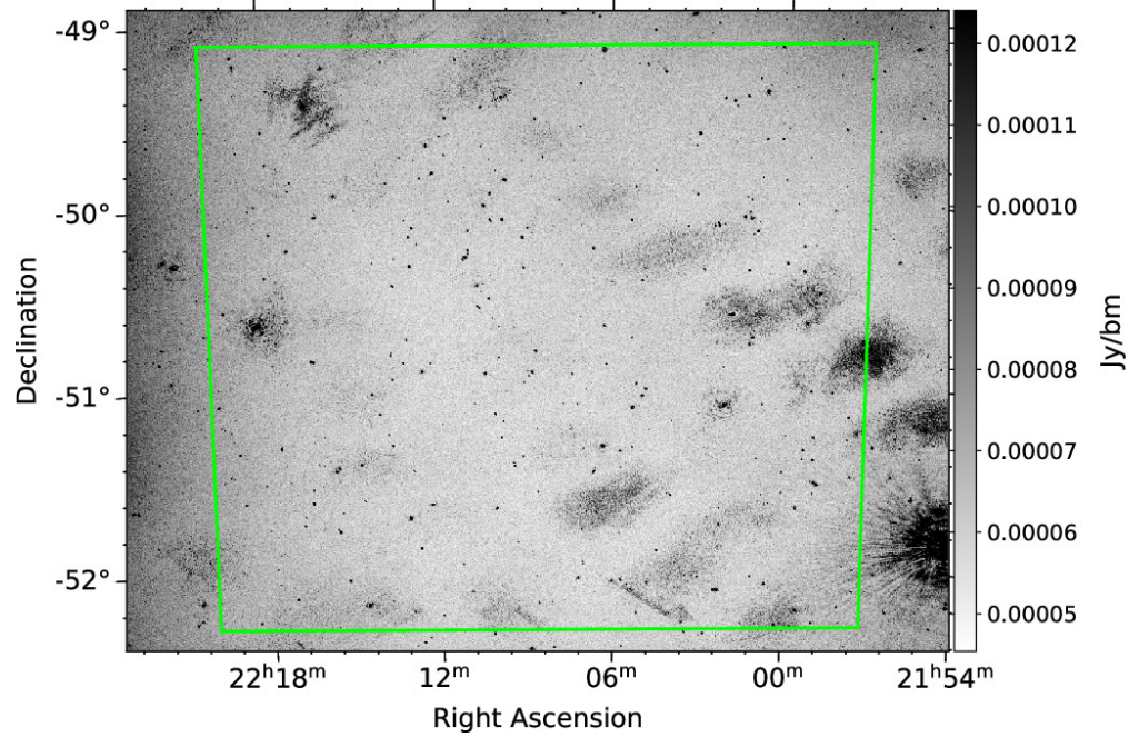
Figure 5. from S. Vanderwoude et al 2024 Astron. J. 167 doi:10.3847/1538-3881/ad2fc8 https://dx.doi.org/10.3847/1538-3881/ad2fc8 © 2024. The Author(s). Published by the American Astronomical Society.
