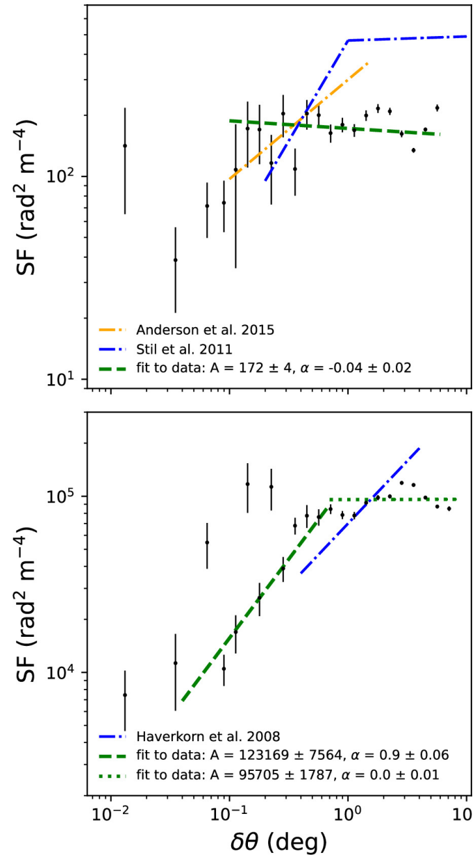
Figure 17. from S. Vanderwoude et al 2024 Astron. J. 167 doi:10.3847/1538-3881/ad2fc8 https://dx.doi.org/10.3847/1538-3881/ad2fc8 © 2024. The Author(s). Published by the American Astronomical Society.
