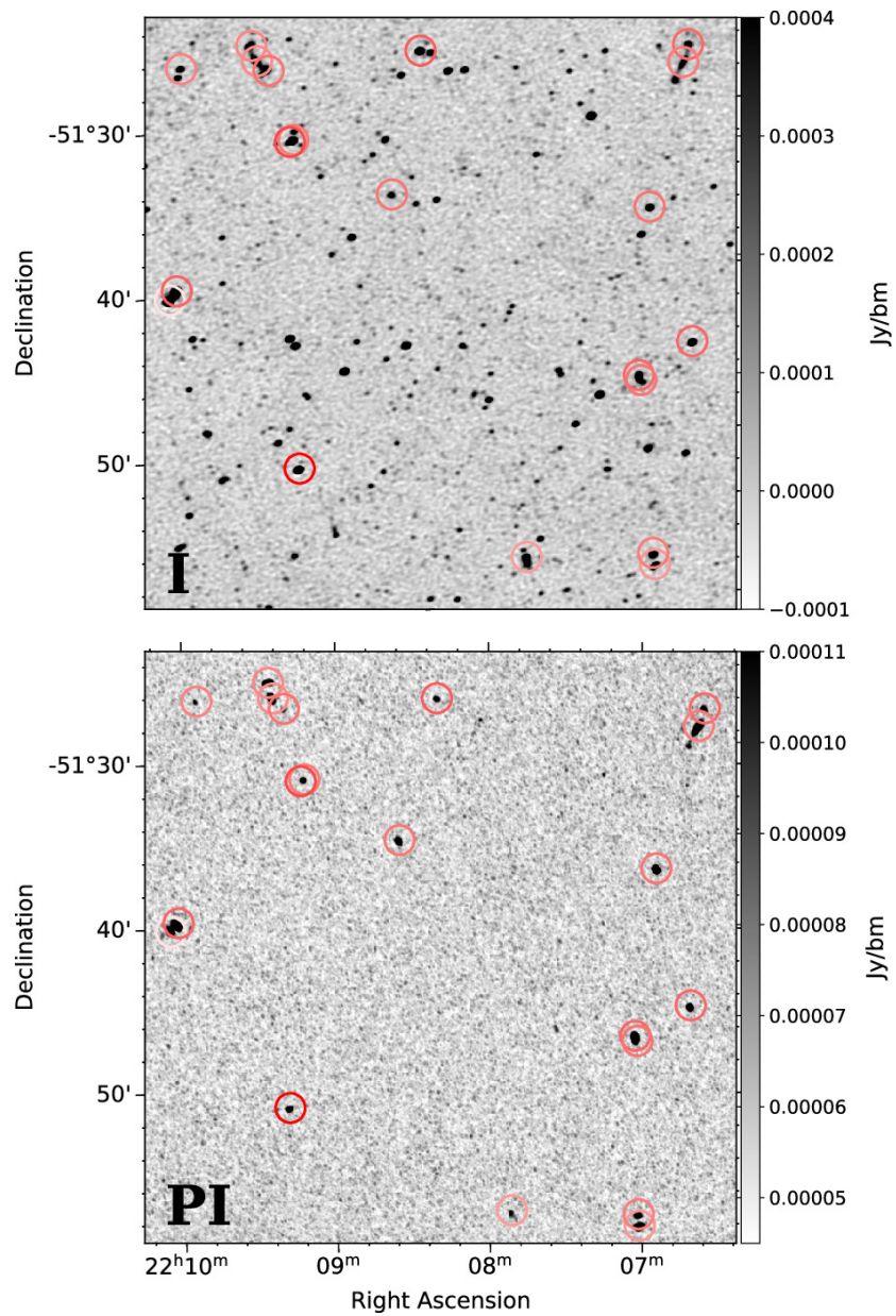
Figure 14. from S. Vanderwoude et al 2024 Astron. J. 167 doi:10.3847/1538-3881/ad2fc8 https://dx.doi.org/10.3847/1538-3881/ad2fc8 © 2024. The Author(s). Published by the American Astronomical Society.
