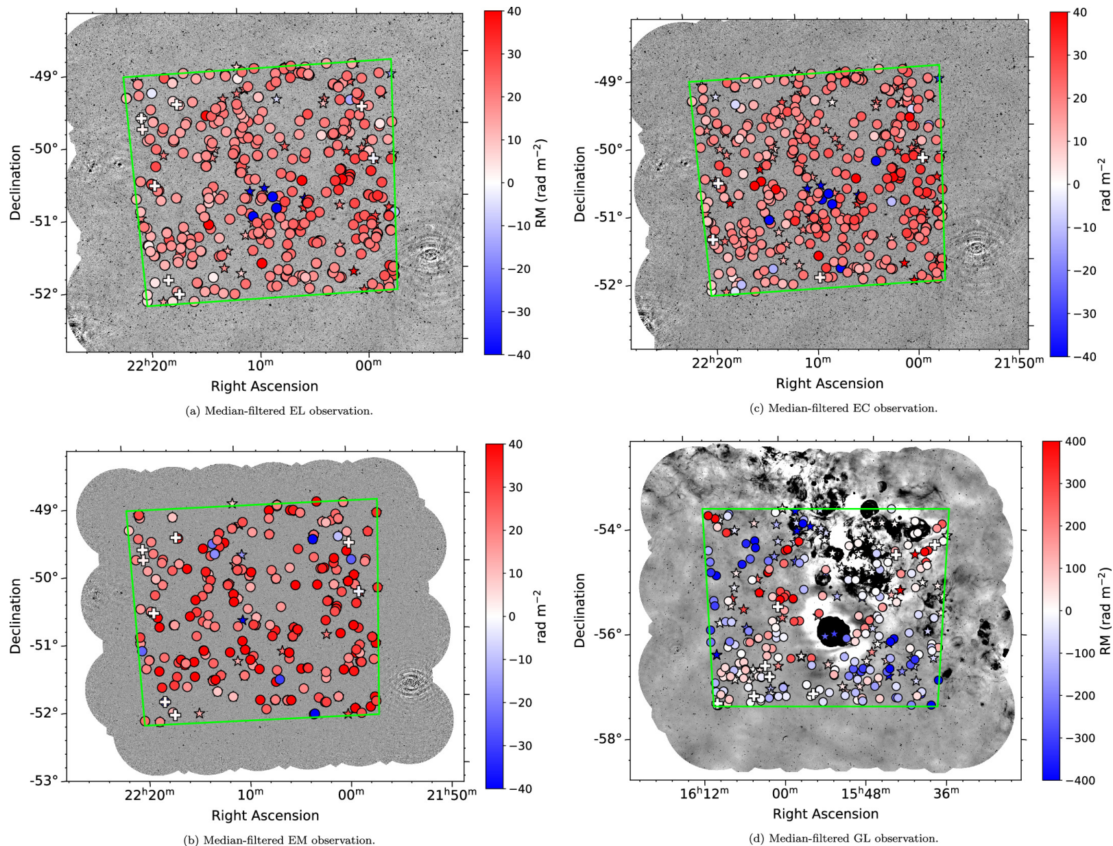
Figure 13. from S. Vanderwoude et al 2024 Astron. J. 167 doi:10.3847/1538-3881/ad2fc8 https://dx.doi.org/10.3847/1538-3881/ad2fc8 © 2024. The Author(s). Published by the American Astronomical Society.
