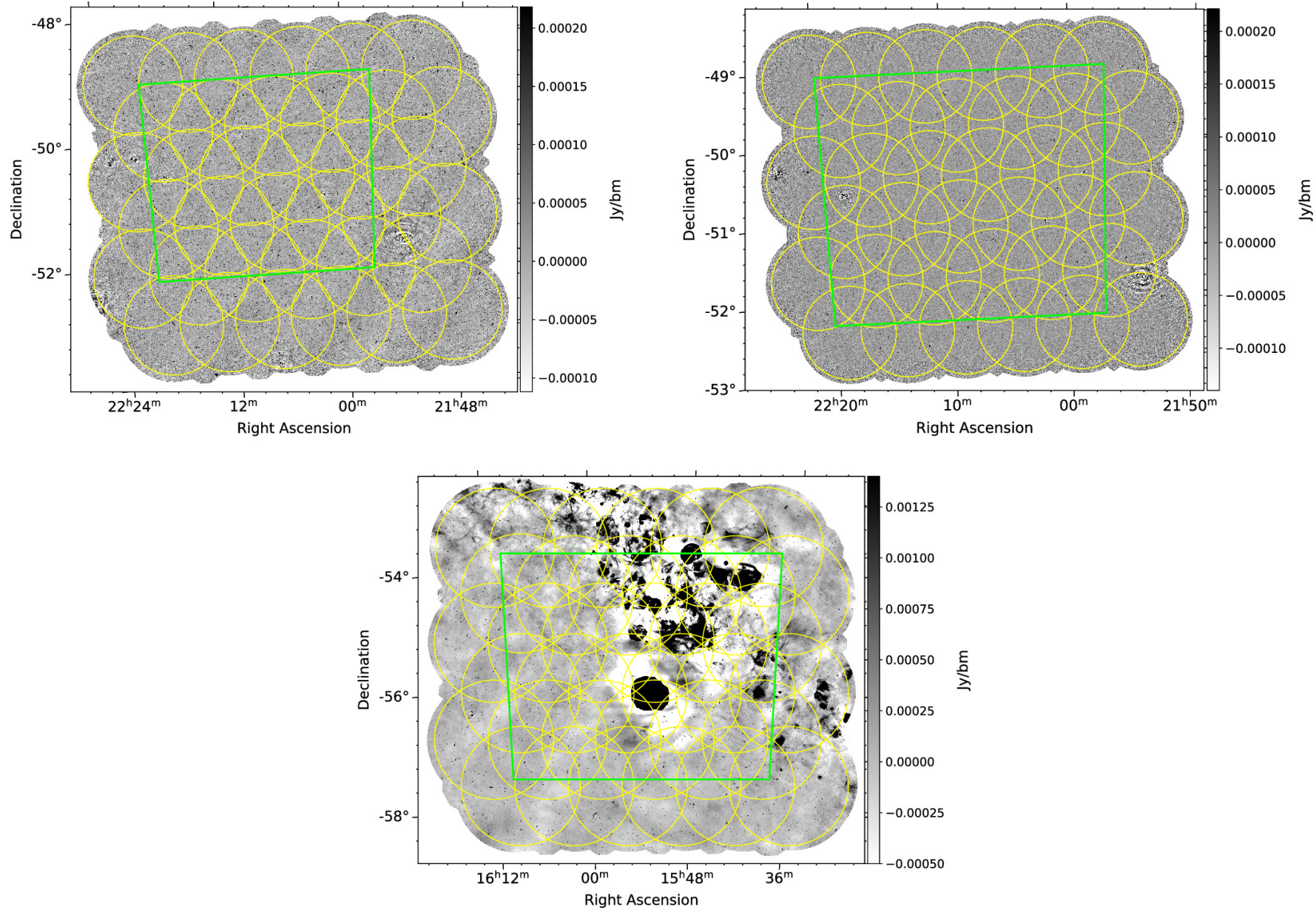
Figure 1. from S. Vanderwoude et al 2024 Astron. J. 167 doi:10.3847/1538-3881/ad2fc8 https://dx.doi.org/10.3847/1538-3881/ad2fc8 © 2024. The Author(s). Published by the American Astronomical Society.
