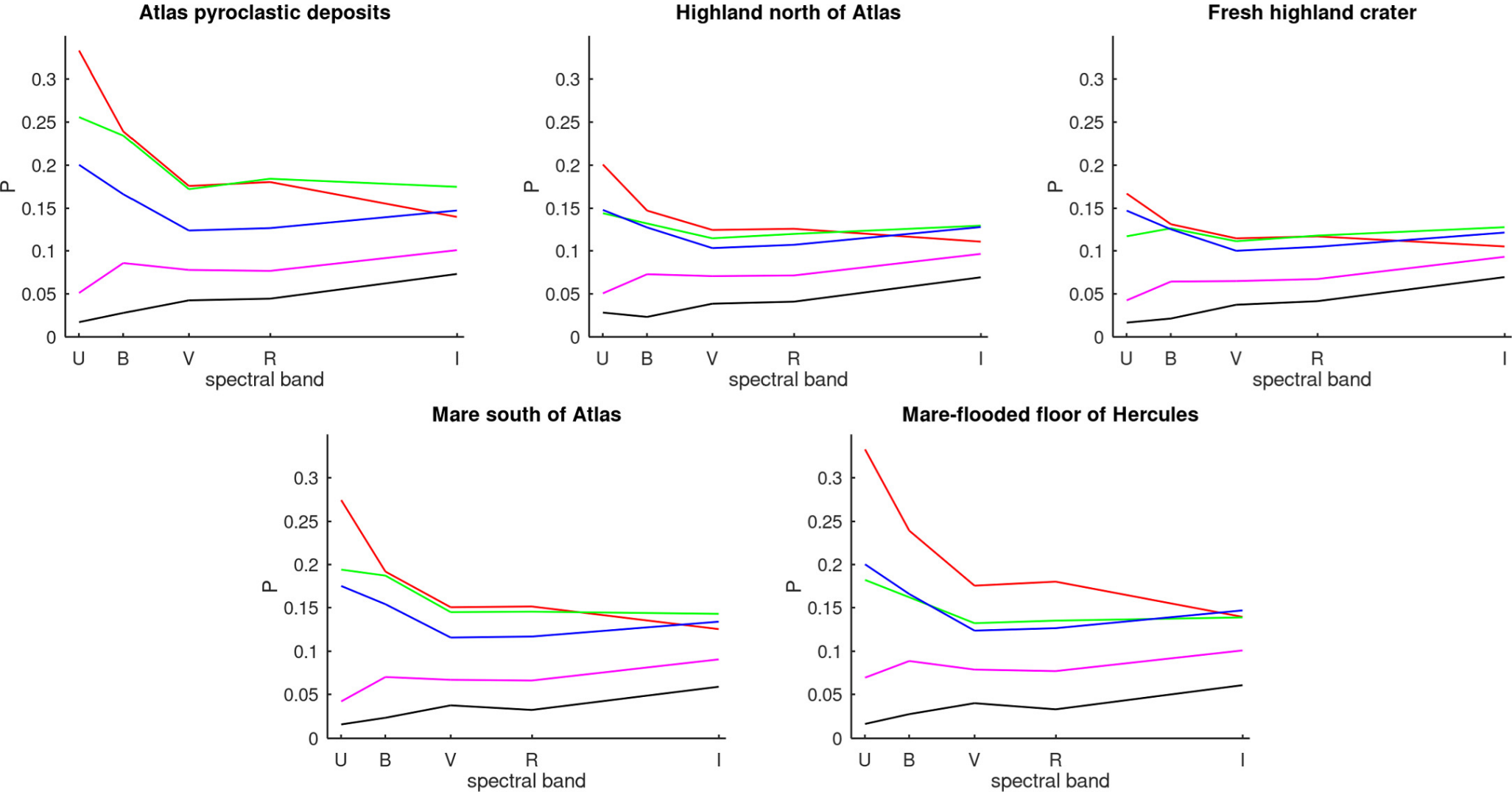
Figure 8. from Christian Wöhler et al 2024 Astron. J. 167 doi:10.3847/1538-3881/ad2f2f https://dx.doi.org/10.3847/1538-3881/ad2f2f © 2024. The Author(s). Published by the American Astronomical Society.
