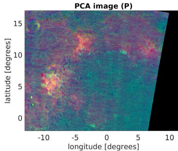
Figure 6. from Christian Wöhler et al 2024 Astron. J. 167 doi:10.3847/1538-3881/ad2f2f https://dx.doi.org/10.3847/1538-3881/ad2f2f © 2024. The Author(s). Published by the American Astronomical Society.
