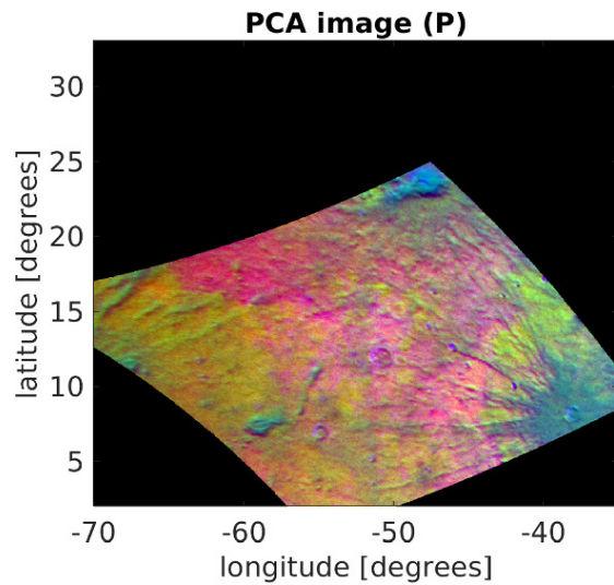
Figure 6. from Christian Wöhler et al 2024 Astron. J. 167 doi:10.3847/1538-3881/ad2f2f https://dx.doi.org/10.3847/1538-3881/ad2f2f © 2024. The Author(s). Published by the American Astronomical Society.
