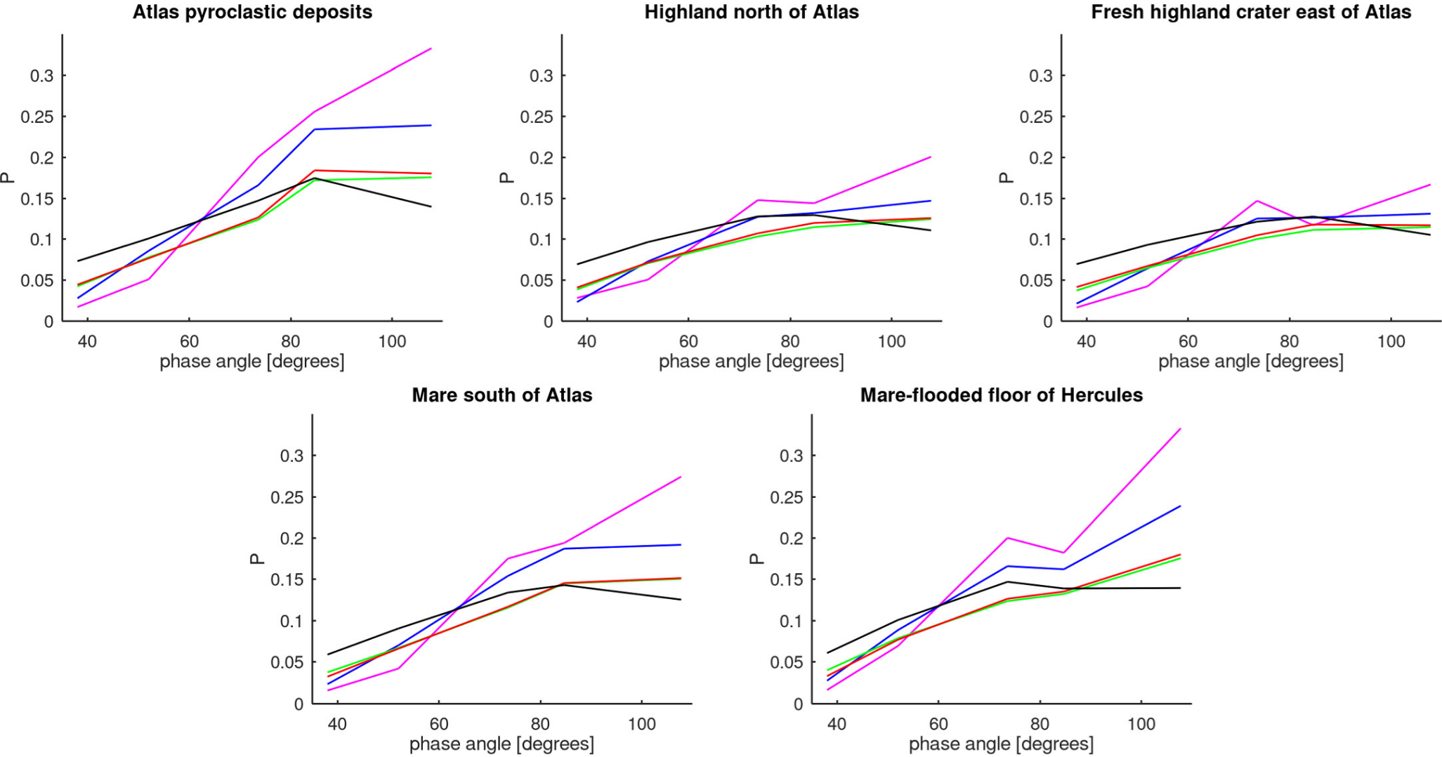
Figure 10. from Christian Wöhler et al 2024 Astron. J. 167 doi:10.3847/1538-3881/ad2f2f https://dx.doi.org/10.3847/1538-3881/ad2f2f © 2024. The Author(s). Published by the American Astronomical Society.
