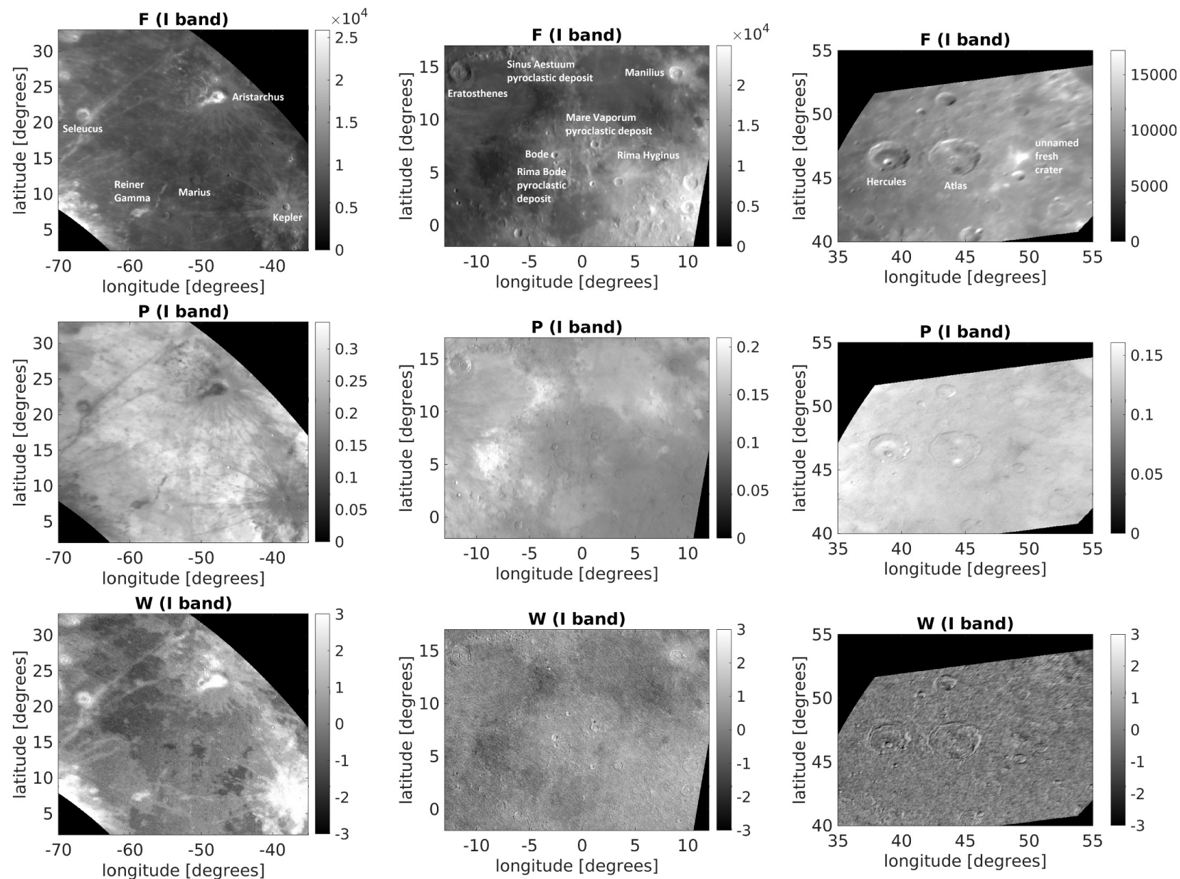
Figure 1. from Christian Wöhler et al 2024 Astron. J. 167 doi:10.3847/1538-3881/ad2f2f https://dx.doi.org/10.3847/1538-3881/ad2f2f © 2024. The Author(s). Published by the American Astronomical Society.
