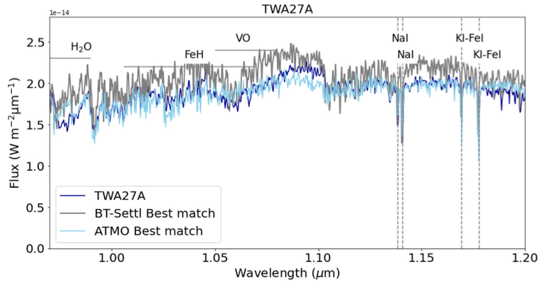
Figure 9. from Elena Manjavacas et al 2024 Astron. J. 167 doi:10.3847/1538-3881/ad2938 https://dx.doi.org/10.3847/1538-3881/ad2938 © 2024. The Author(s). Published by the American Astronomical Society.
