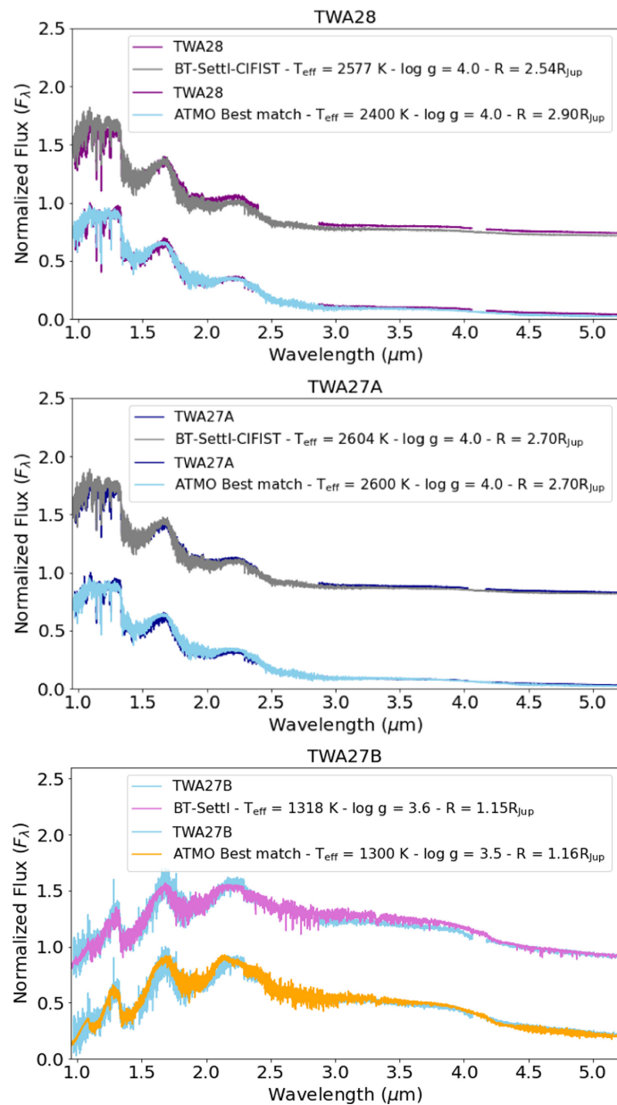
Figure 6. from Elena Manjavacas et al 2024 Astron. J. 167 doi:10.3847/1538-3881/ad2938 https://dx.doi.org/10.3847/1538-3881/ad2938 © 2024. The Author(s). Published by the American Astronomical Society.
