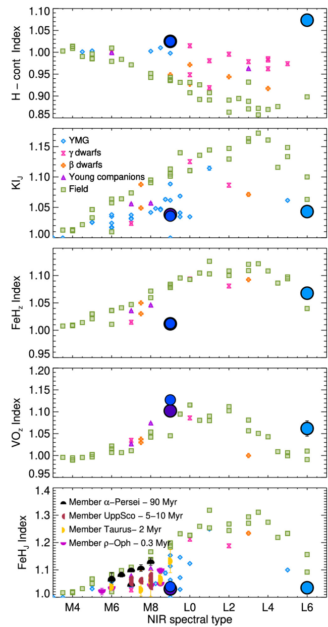
Figure 4. from Elena Manjavacas et al 2024 Astron. J. 167 doi:10.3847/1538-3881/ad2938 https://dx.doi.org/10.3847/1538-3881/ad2938 © 2024. The Author(s). Published by the American Astronomical Society.
