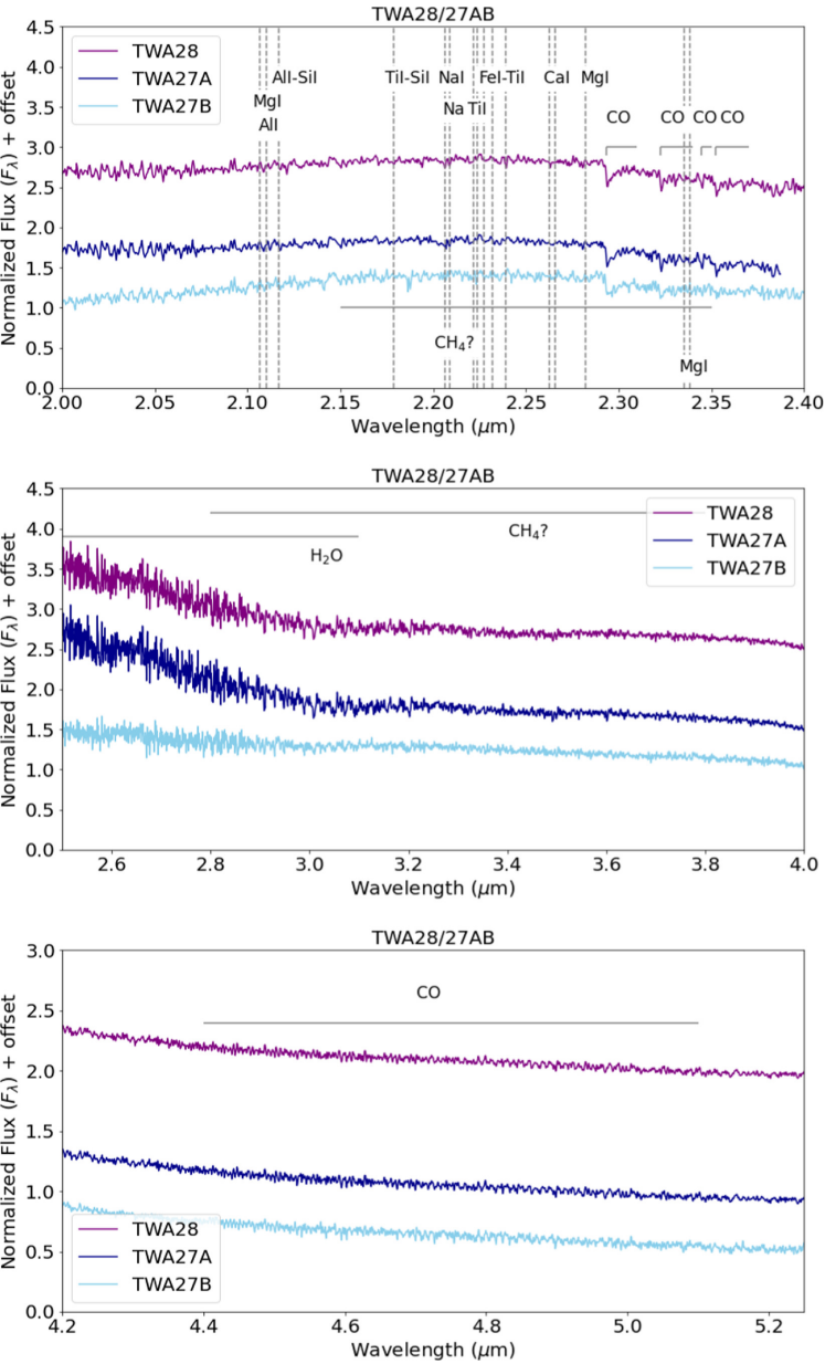
Figure 3. from Elena Manjavacas et al 2024 Astron. J. 167 doi:10.3847/1538-3881/ad2938 https://dx.doi.org/10.3847/1538-3881/ad2938 © 2024. The Author(s). Published by the American Astronomical Society.
