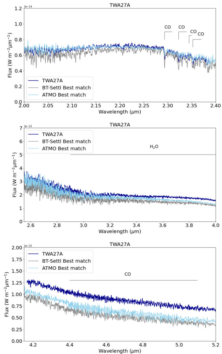
Figure 10. from Elena Manjavacas et al 2024 Astron. J. 167 doi:10.3847/1538-3881/ad2938 https://dx.doi.org/10.3847/1538-3881/ad2938 © 2024. The Author(s). Published by the American Astronomical Society.
