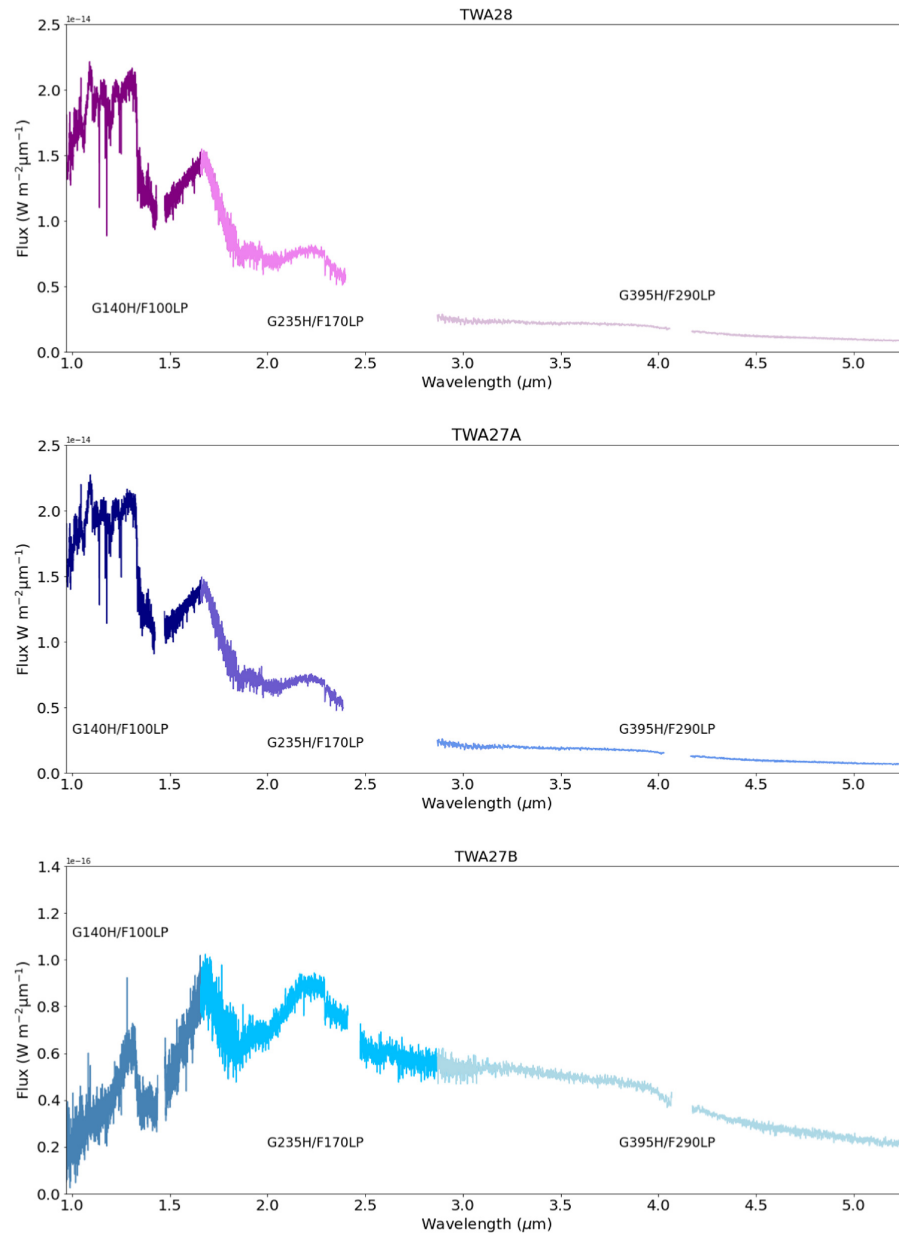
Figure 1. from Elena Manjavacas et al 2024 Astron. J. 167 doi:10.3847/1538-3881/ad2938 https://dx.doi.org/10.3847/1538-3881/ad2938 © 2024. The Author(s). Published by the American Astronomical Society.
