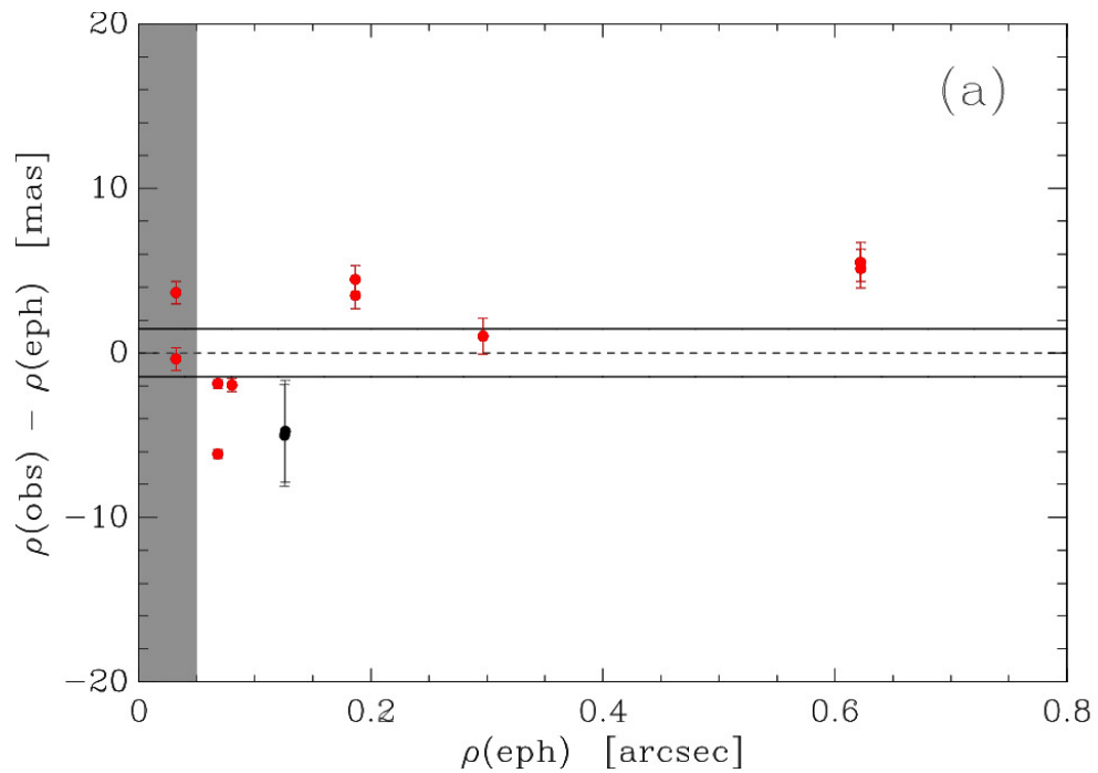
Figure 8. from James W. Davidson et al 2024 Astron. J. 167 doi:10.3847/1538-3881/ad1ff6 https://dx.doi.org/10.3847/1538-3881/ad1ff6 © 2024. The Author(s). Published by the American Astronomical Society.
