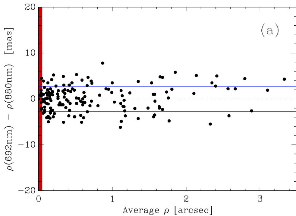
Figure 7. from James W. Davidson et al 2024 Astron. J. 167 doi:10.3847/1538-3881/ad1ff6 https://dx.doi.org/10.3847/1538-3881/ad1ff6 © 2024. The Author(s). Published by the American Astronomical Society.
