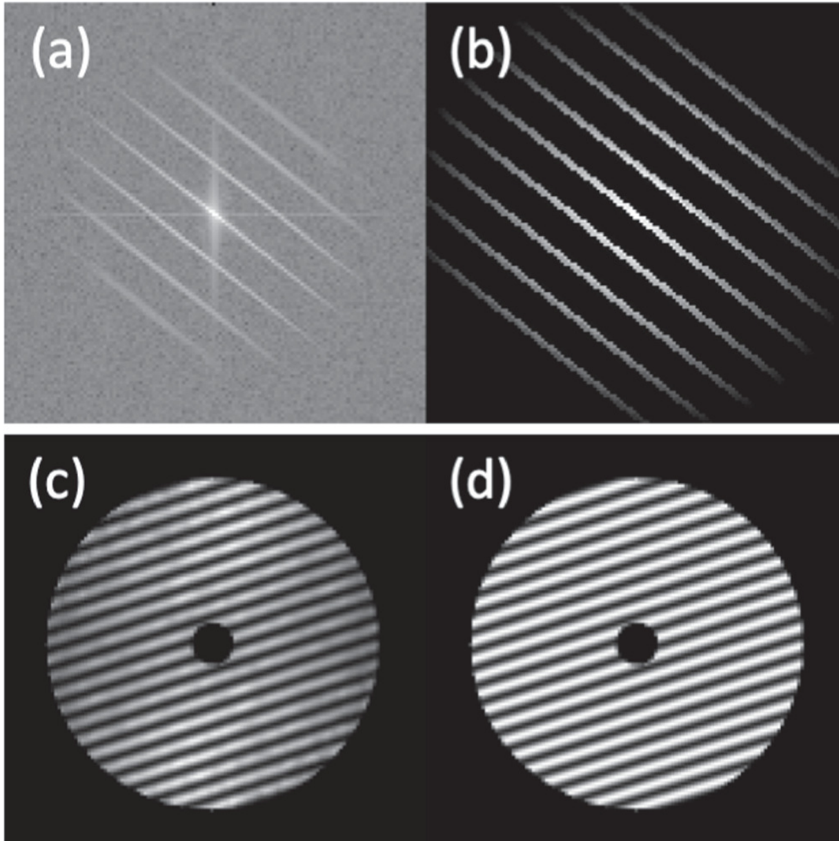
Figure 5. from James W. Davidson et al 2024 Astron. J. 167 doi:10.3847/1538-3881/ad1ff6 https://dx.doi.org/10.3847/1538-3881/ad1ff6 © 2024. The Author(s). Published by the American Astronomical Society.
