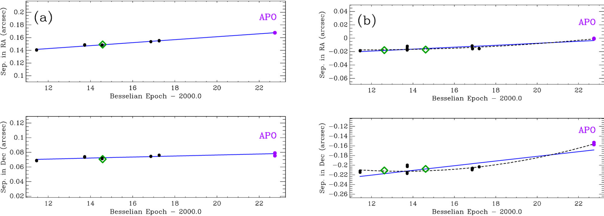
Figure 13. from James W. Davidson et al 2024 Astron. J. 167 doi:10.3847/1538-3881/ad1ff6 https://dx.doi.org/10.3847/1538-3881/ad1ff6 © 2024. The Author(s). Published by the American Astronomical Society.
