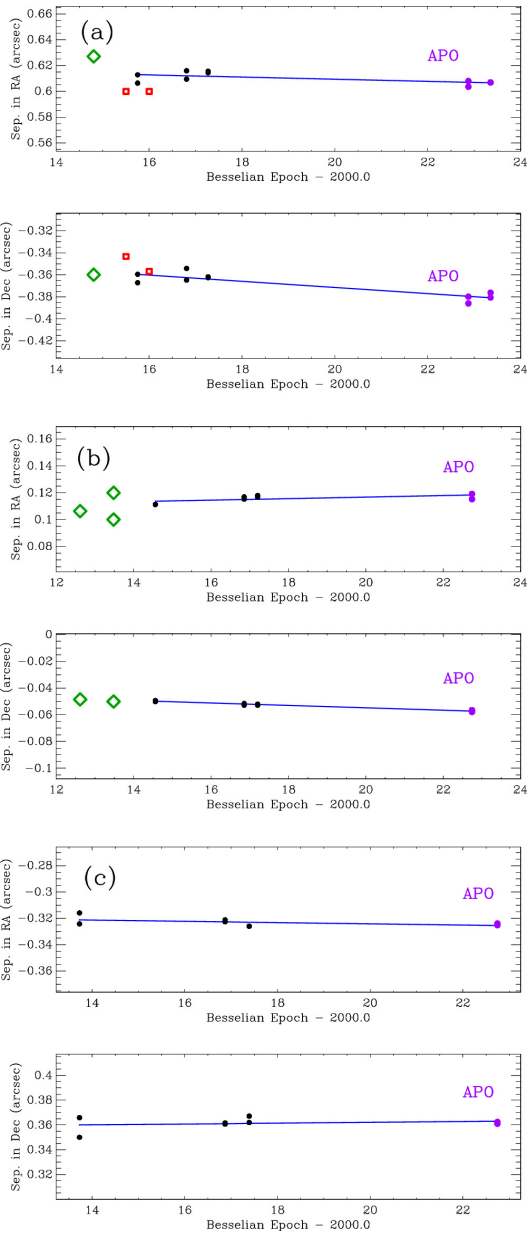
Figure 12. from James W. Davidson et al 2024 Astron. J. 167 doi:10.3847/1538-3881/ad1ff6 https://dx.doi.org/10.3847/1538-3881/ad1ff6 © 2024. The Author(s). Published by the American Astronomical Society.
