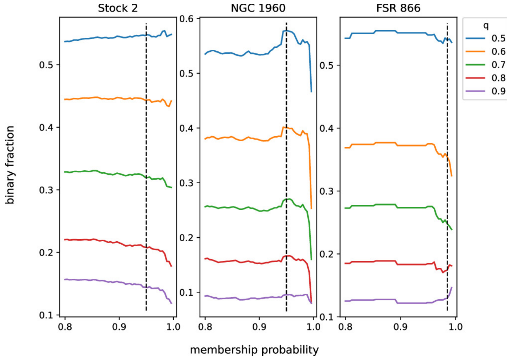
Figure 8. from L. Yalyalieva et al 2024 Astron. J. 167 doi:10.3847/1538-3881/ad1ff0 https://dx.doi.org/10.3847/1538-3881/ad1ff0 © 2024. The Author(s). Published by the American Astronomical Society.
