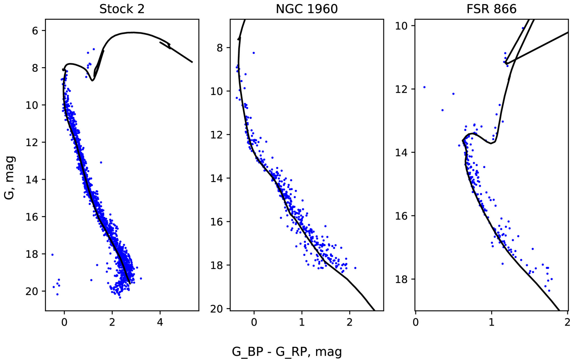
Figure 6. from L. Yalyalieva et al 2024 Astron. J. 167 doi:10.3847/1538-3881/ad1ff0 https://dx.doi.org/10.3847/1538-3881/ad1ff0 © 2024. The Author(s). Published by the American Astronomical Society.
