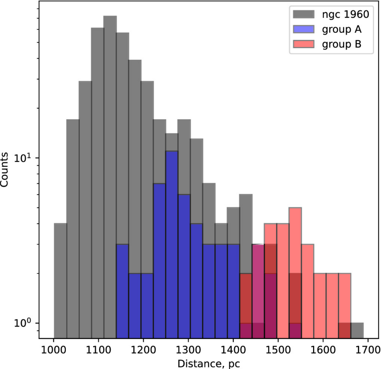
Figure 4. from L. Yalyalieva et al 2024 Astron. J. 167 doi:10.3847/1538-3881/ad1ff0 https://dx.doi.org/10.3847/1538-3881/ad1ff0 © 2024. The Author(s). Published by the American Astronomical Society.
