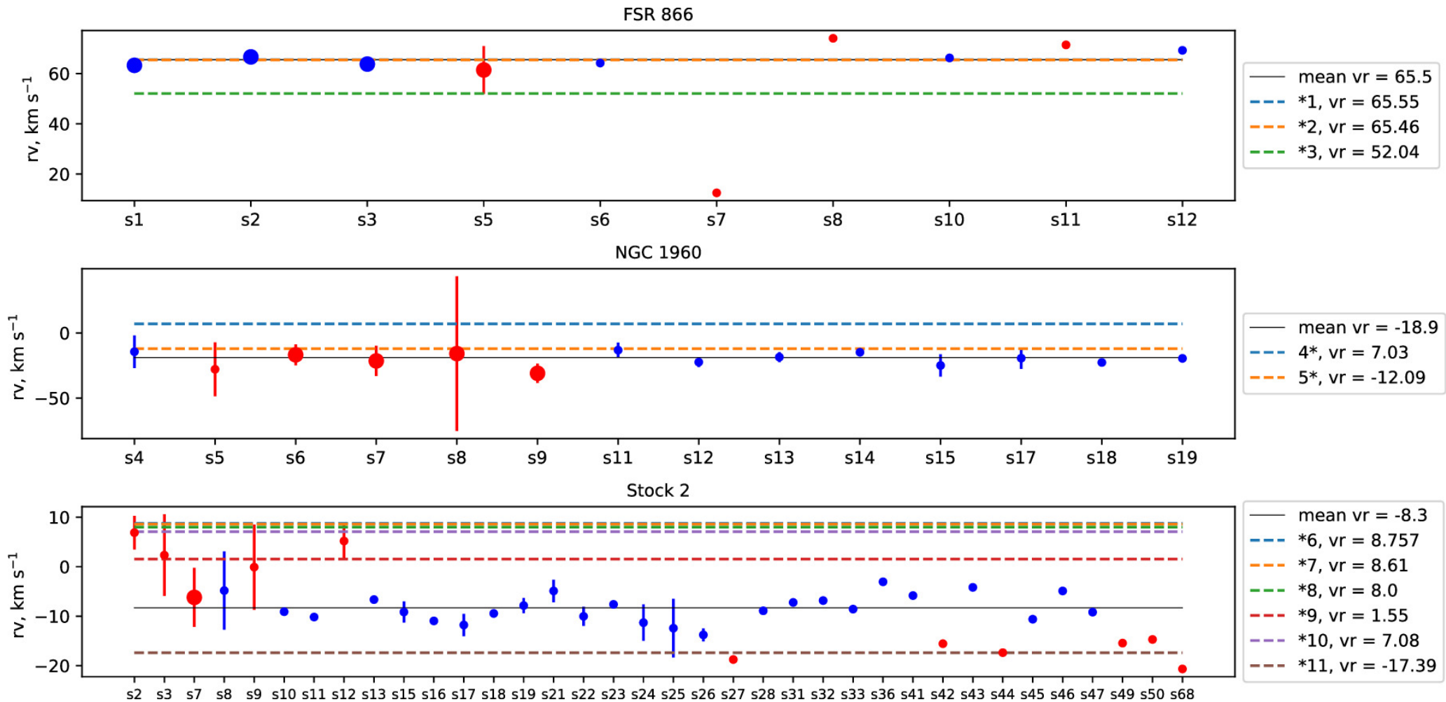
Figure 10. from L. Yalyalieva et al 2024 Astron. J. 167 doi:10.3847/1538-3881/ad1ff0 https://dx.doi.org/10.3847/1538-3881/ad1ff0 © 2024. The Author(s). Published by the American Astronomical Society.
