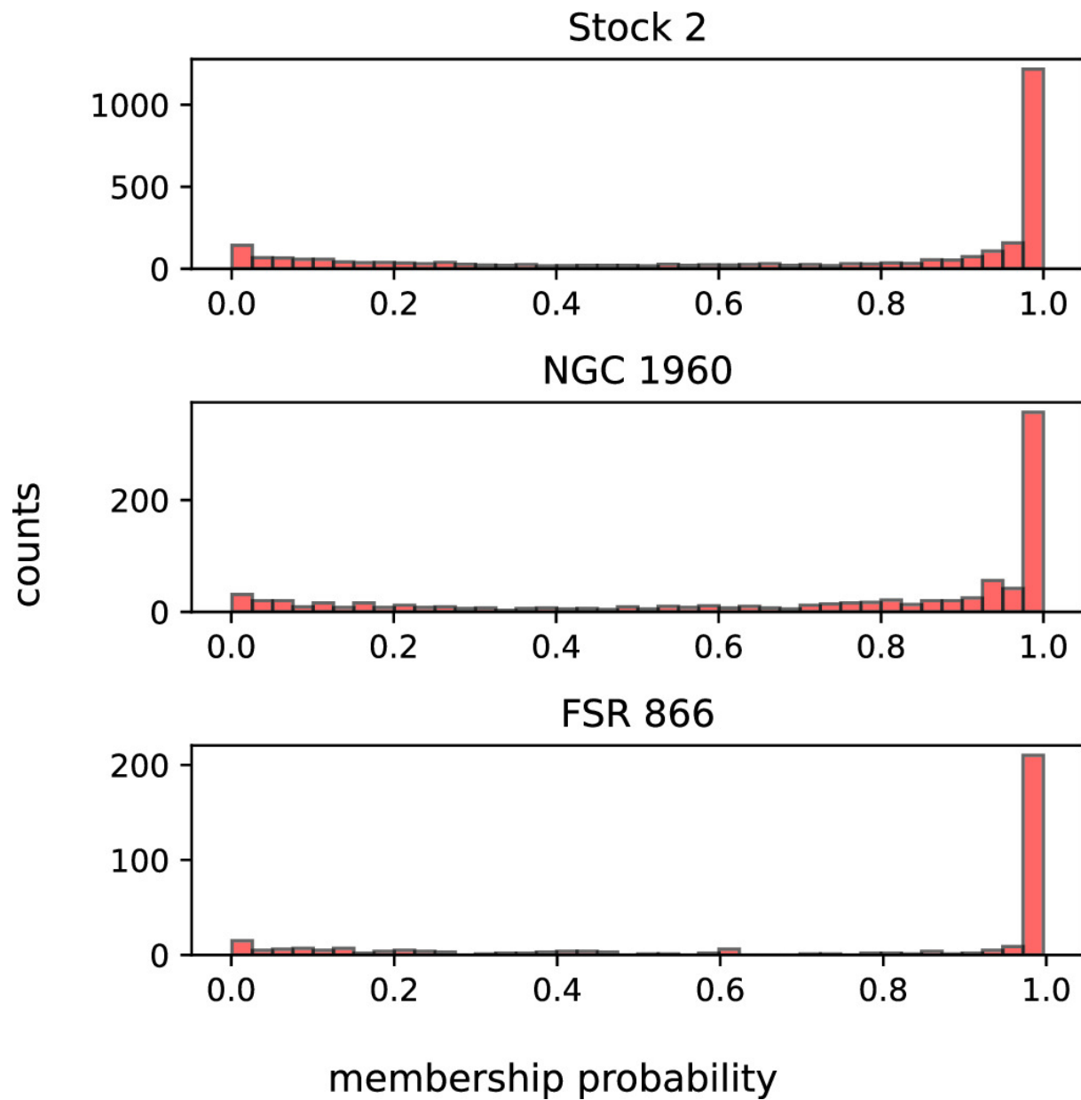
Figure 1. from L. Yalyalieva et al 2024 Astron. J. 167 doi:10.3847/1538-3881/ad1ff0 https://dx.doi.org/10.3847/1538-3881/ad1ff0 © 2024. The Author(s). Published by the American Astronomical Society.
