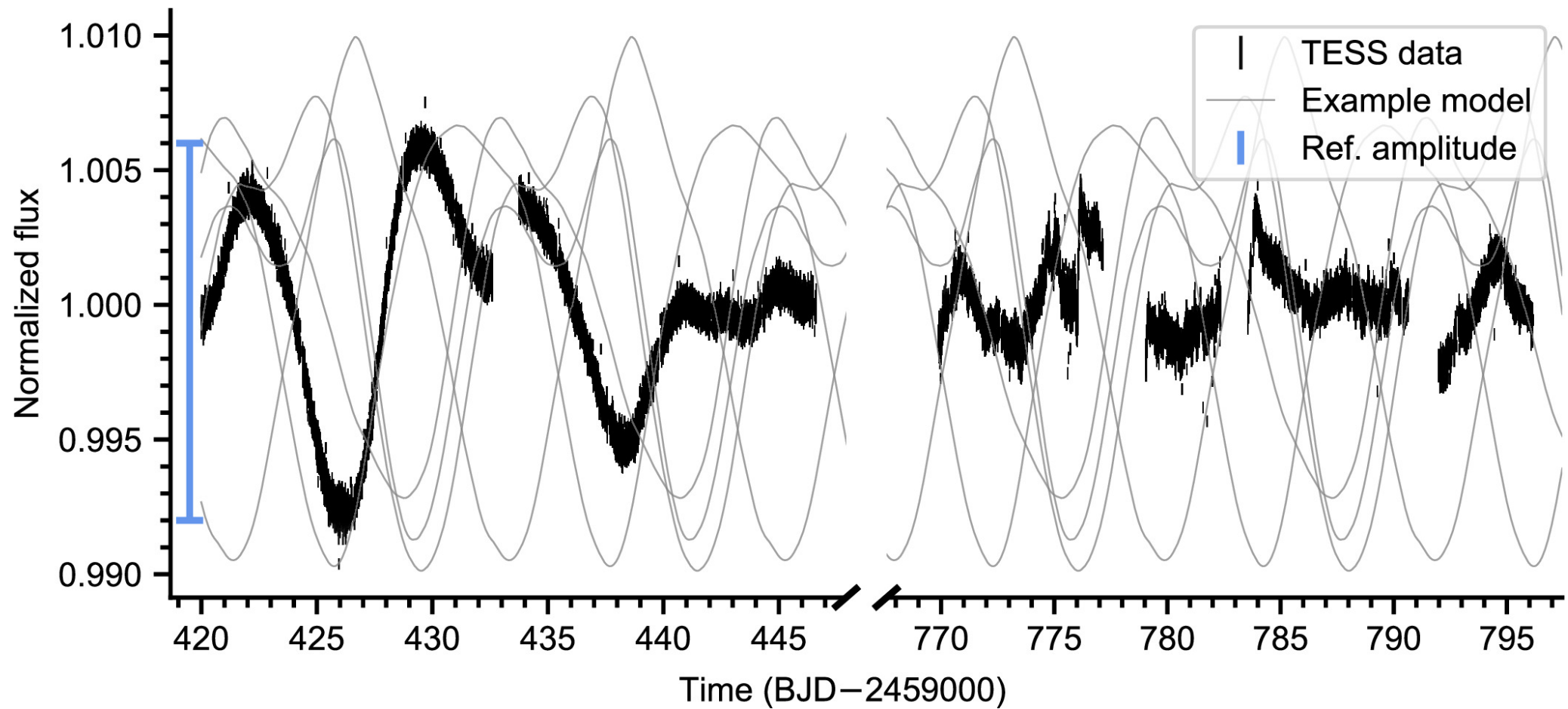
Figure 5. from Isaac S. Narrett et al 2024 Astron. J. 167 doi:10.3847/1538-3881/ad1f6c https://dx.doi.org/10.3847/1538-3881/ad1f6c © 2024. The Author(s). Published by the American Astronomical Society.
