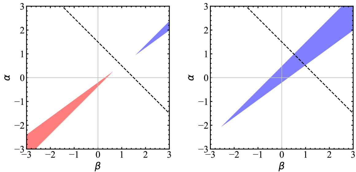
(a) Kepler-223
