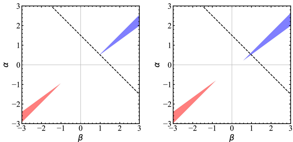
(c) Kepler-80
