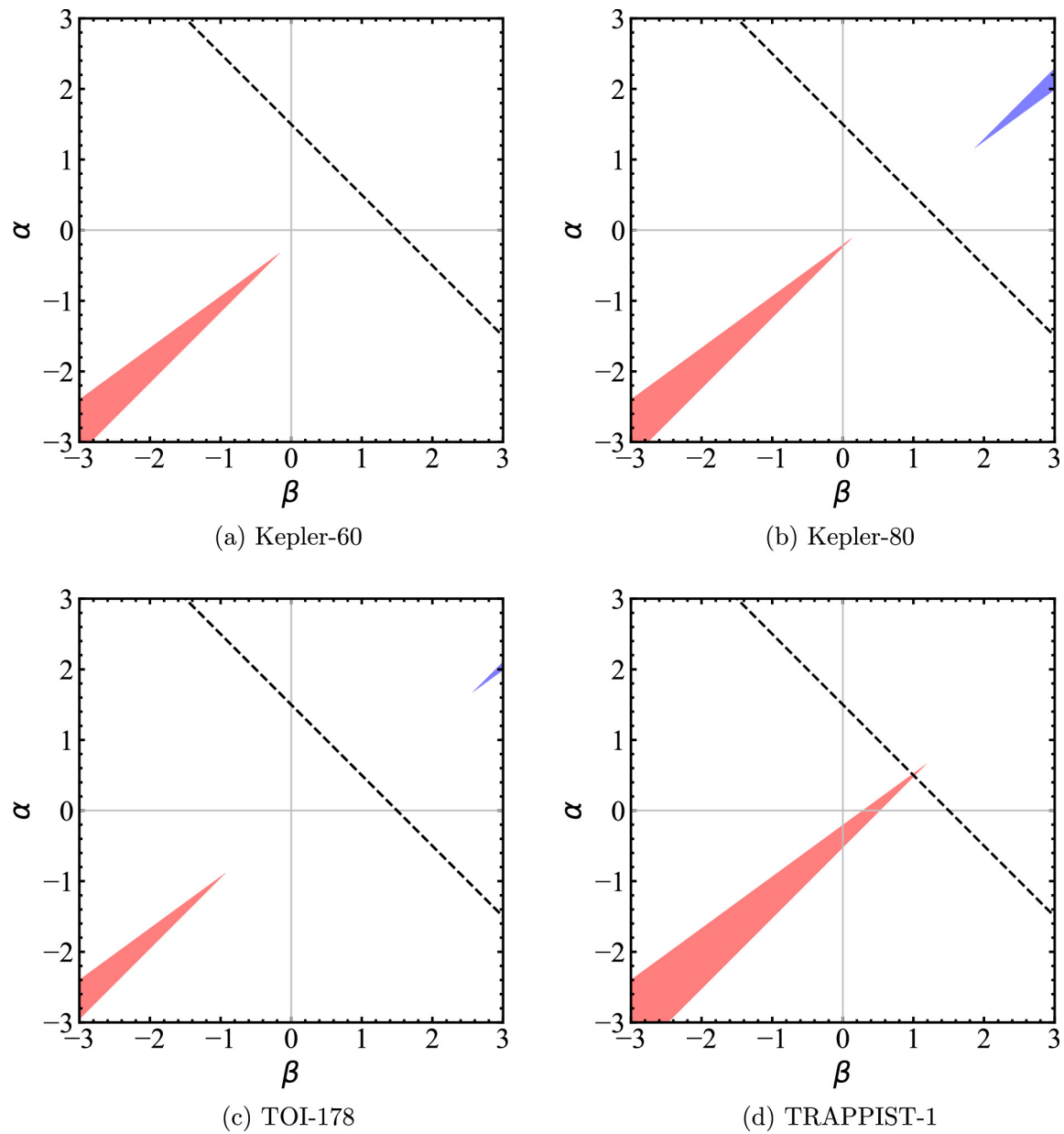
Figure 8. from Ka Ho Wong and Man Hoi Lee 2024 Astron. J. 167 doi:10.3847/1538-3881/ad1f60 https://dx.doi.org/10.3847/1538-3881/ad1f60 © 2024. The Author(s). Published by the American Astronomical Society.
