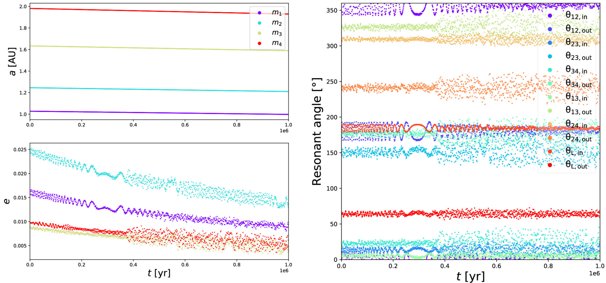
Figure 7. from Ka Ho Wong and Man Hoi Lee 2024 Astron. J. 167 doi:10.3847/1538-3881/ad1f60 https://dx.doi.org/10.3847/1538-3881/ad1f60 © 2024. The Author(s). Published by the American Astronomical Society.
