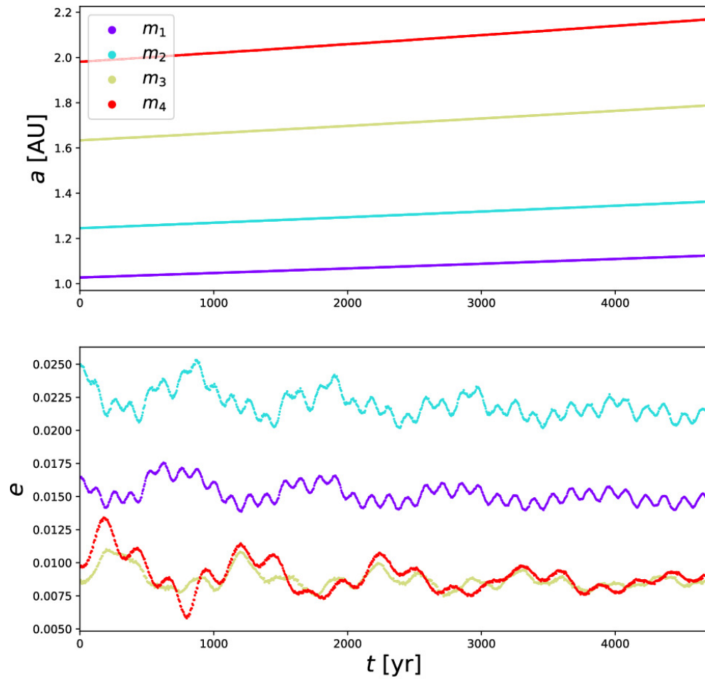
Figure 6. from Ka Ho Wong and Man Hoi Lee 2024 Astron. J. 167 doi:10.3847/1538-3881/ad1f60 https://dx.doi.org/10.3847/1538-3881/ad1f60 © 2024. The Author(s). Published by the American Astronomical Society.
