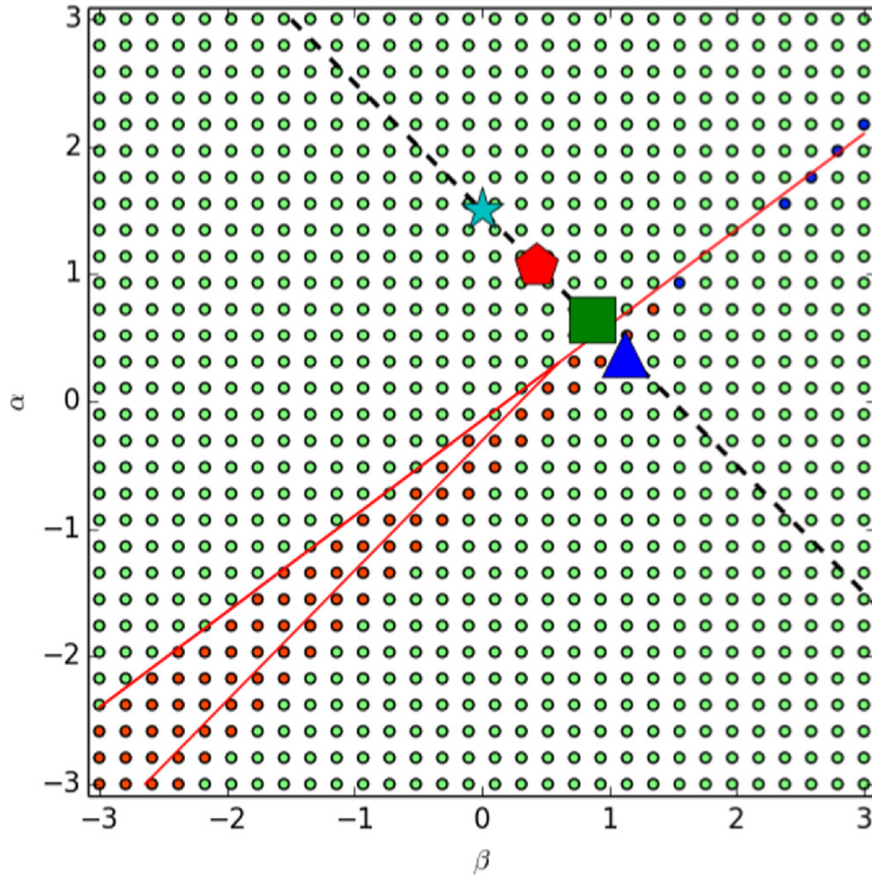
Figure 5. from Ka Ho Wong and Man Hoi Lee 2024 Astron. J. 167 doi:10.3847/1538-3881/ad1f60 https://dx.doi.org/10.3847/1538-3881/ad1f60 © 2024. The Author(s). Published by the American Astronomical Society.
