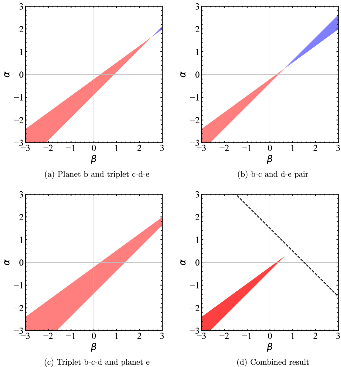
Figure 4. from Ka Ho Wong and Man Hoi Lee 2024 Astron. J. 167 doi:10.3847/1538-3881/ad1f60 https://dx.doi.org/10.3847/1538-3881/ad1f60 © 2024. The Author(s). Published by the American Astronomical Society.
